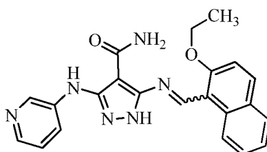
5-(((2-ethoxynaphthalen-1-yl)methylene)amino)-3-(pyridin-3-ylamino)-1H-pyrazole-4-carboxamide
