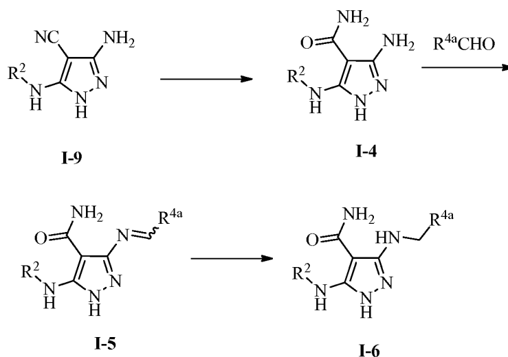
Scheme III
