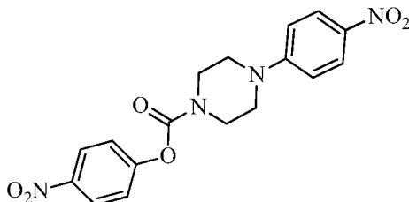
4-nitrophenyl 4-(4-nitrophenyl)piperazine-1-carboxylate
