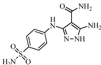
5-amino-3-((4-sulfamoylphenyl)amino)-1H-pyrazole-4-carboxamide
