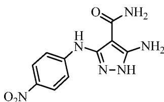
5-amino-3-((4-nitrophenyl)amino)-1H-pyrazole-4-carboxamide
