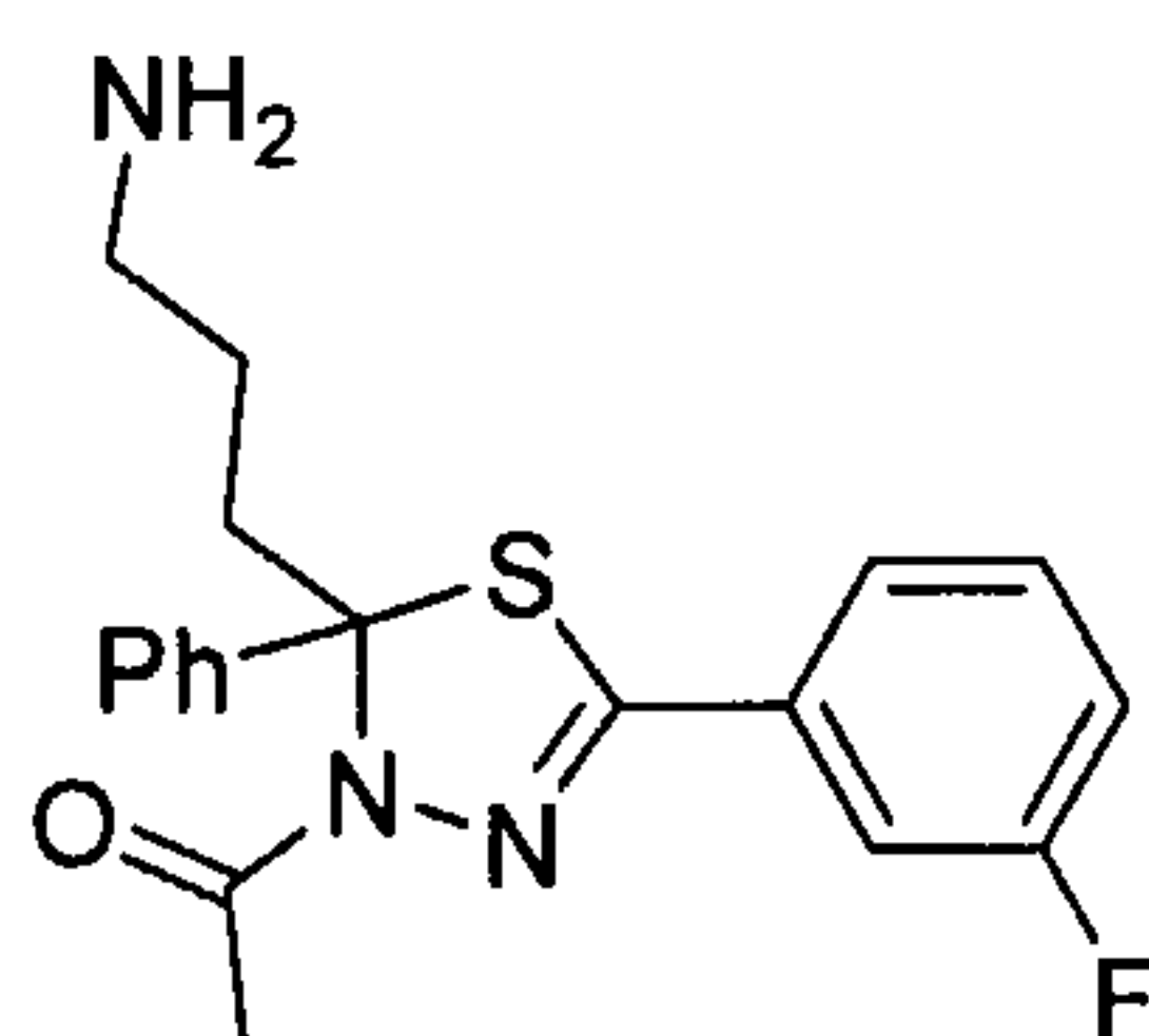
Synthesis of 1-(2-(3-aminopropyl)-5-(3-fluorophenyl)-2-phenyl-1,3,4-thiadiazol-3(2H)-yl)ethanone
