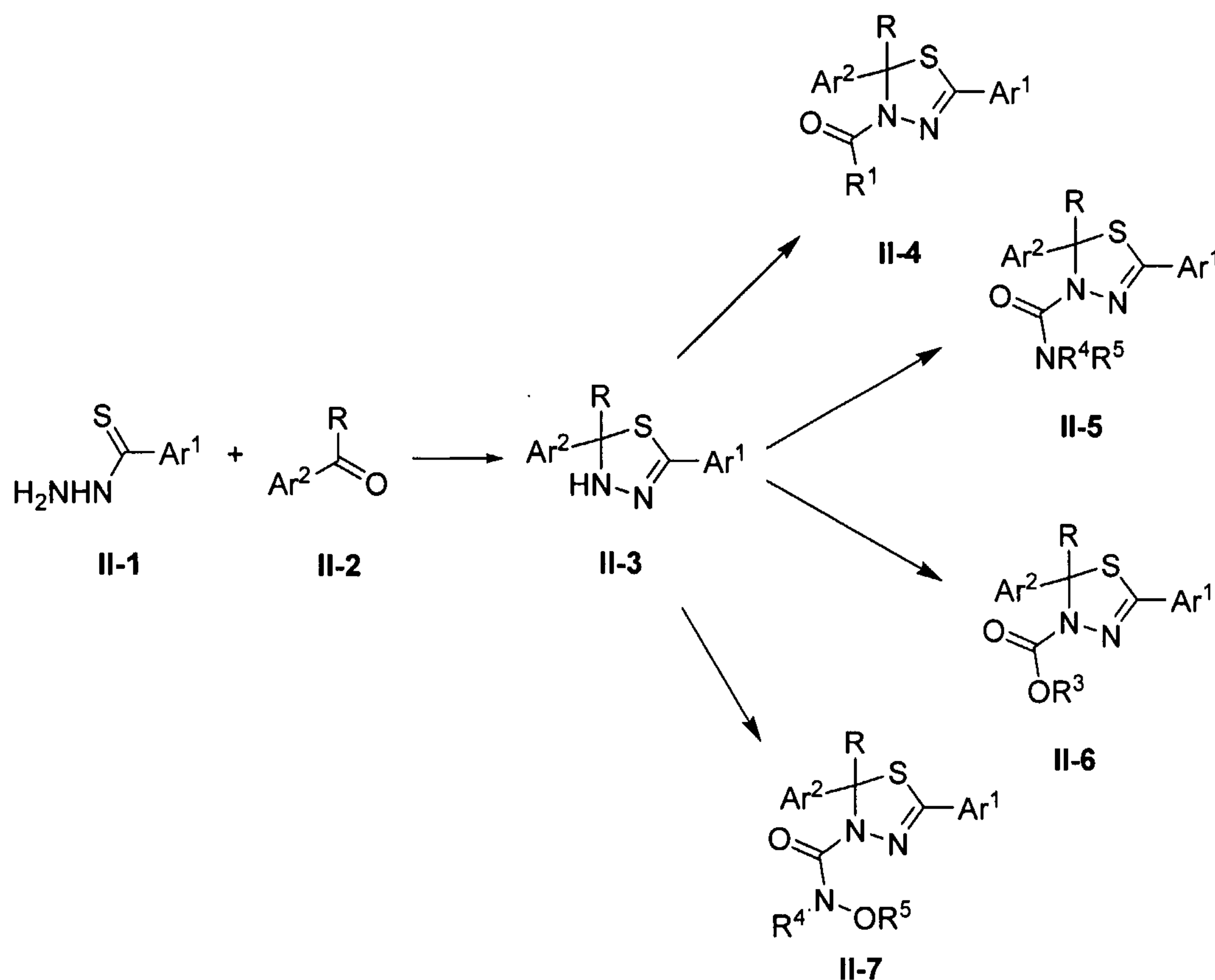
Scheme II
