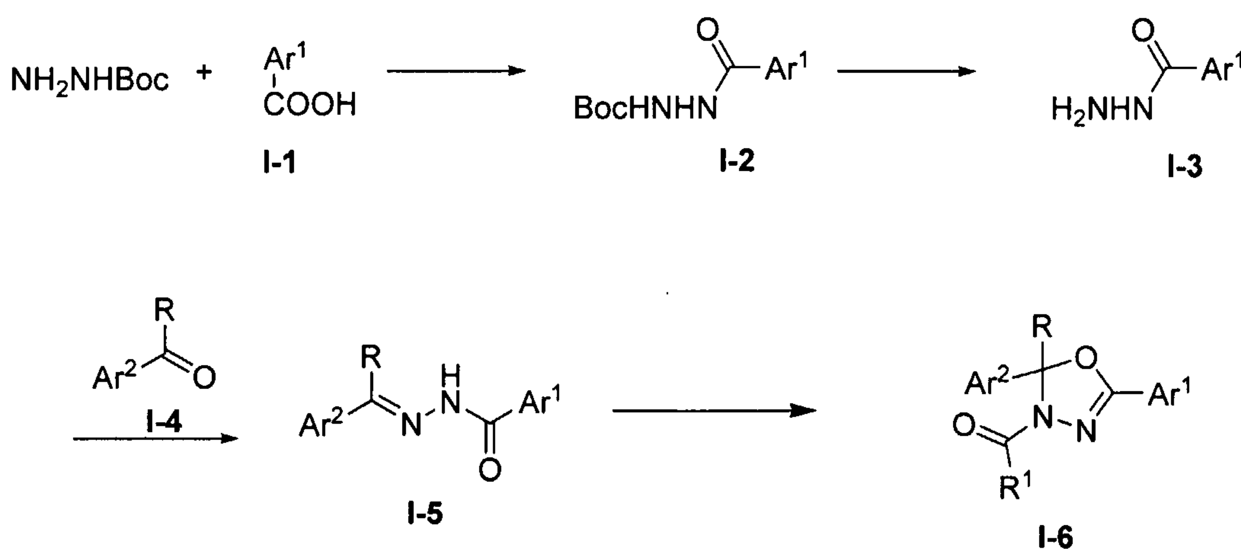
Scheme I
