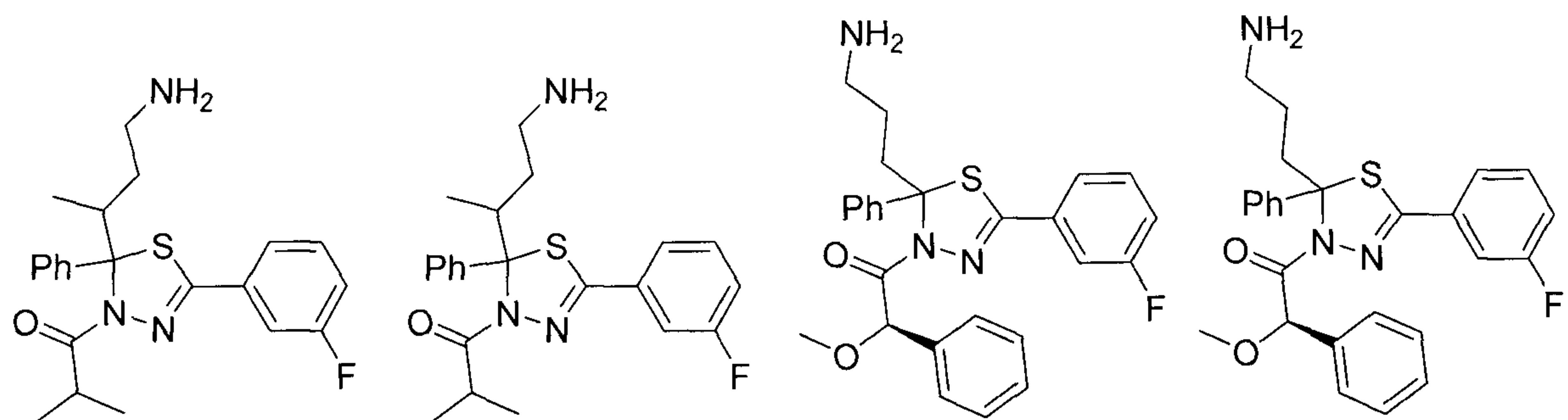
(Diastereomer pair A) (Diastereomer pair B) (Diastereomer A) (Diastereomer B)
