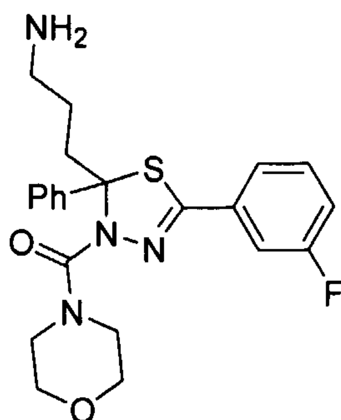
[2-(3-Aminopropyl)-5-(3-fluorophenyl)-2-phenyl-[1,3,4]thiadiazol-3-yl]-morpholin-4-yl-methanone
