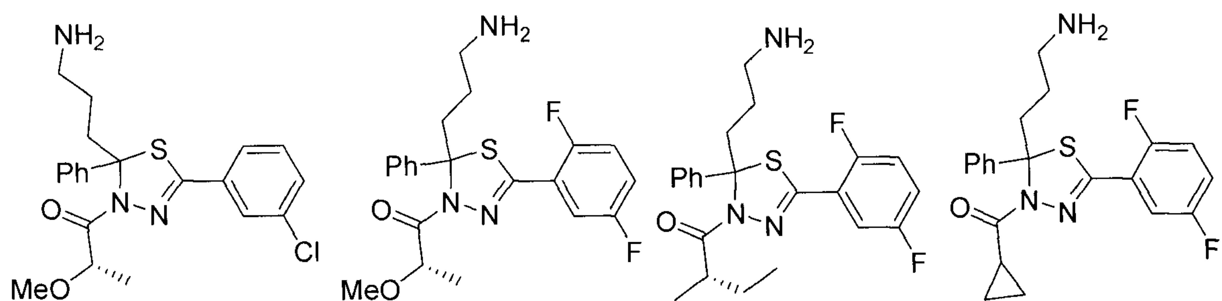
(Diastereomer A) (Diastereomer B)
