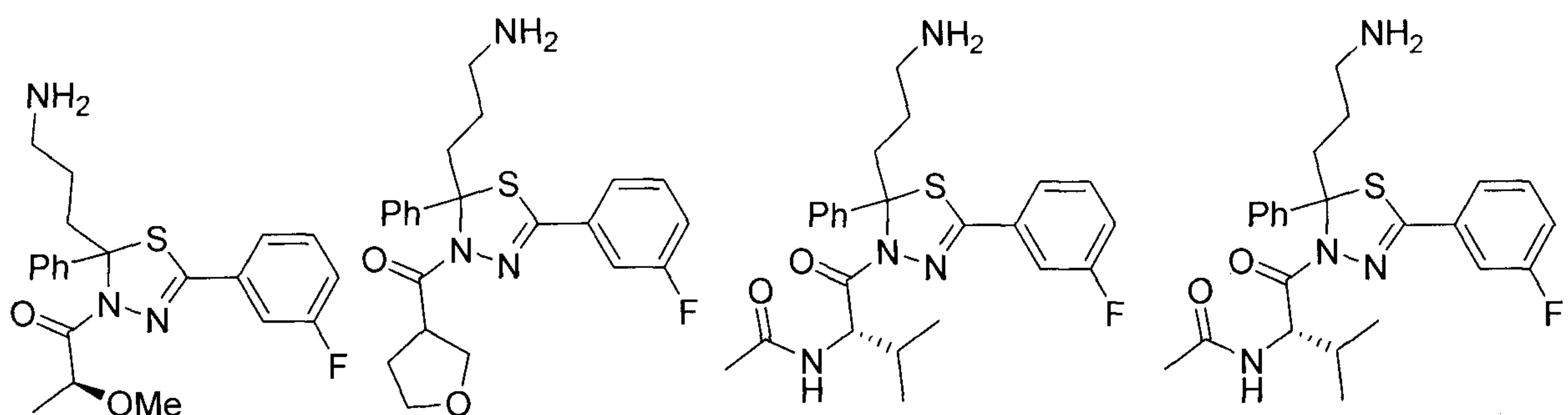
(Diastereomer A) (Diastereomer B)
