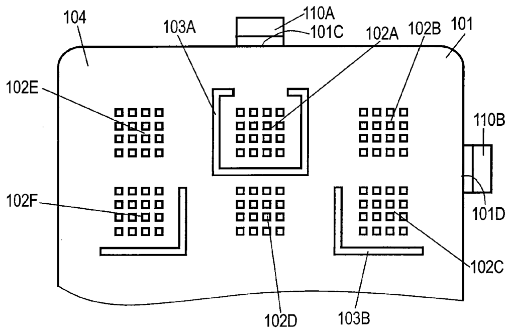
FIG. 13 PRIOR ART
