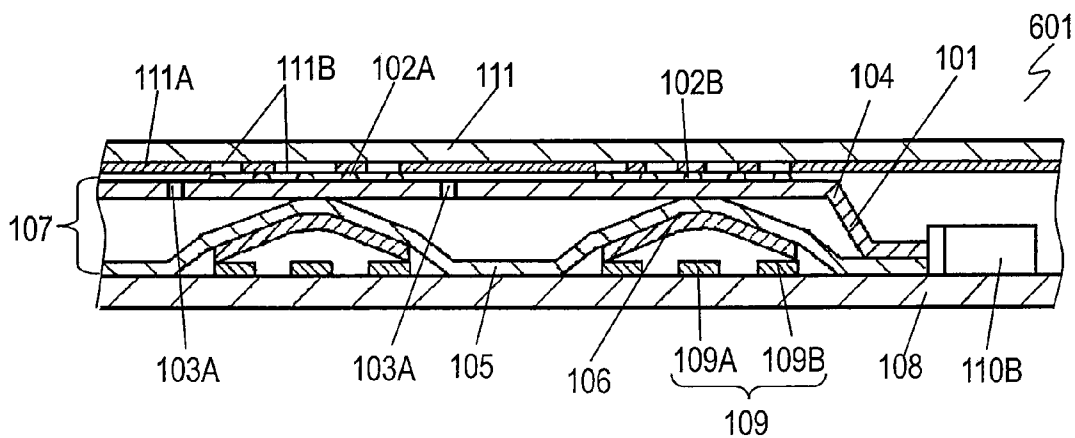
FIG. 11 PRIOR ART
