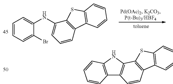
Synthesis of 12H-benzo[4,5]thieno[2,3-a]carbazole
