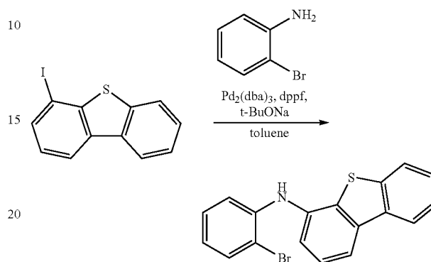
Synthesis of N-(2-bromophenyl)dibenzo[b,d]thiophen-4-amine
