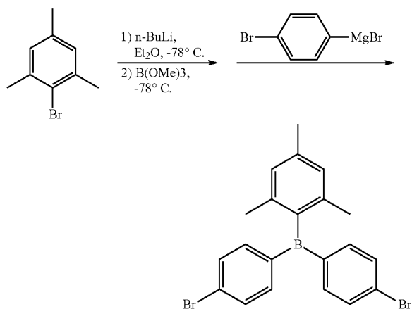
Synthesis of bis(4-bromophenyl)(mesityl)borane
