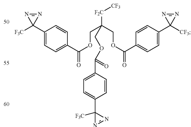
2-(perfluoroethyl)-2-(((4-(3-(trifluoromethyl)-3H-diazirin-3-yl)benzoyl)oxy)methyl)propane-1,3-diyl bis(4-(3-(trifluoromethyl)-3H-diazirin-3-yl)benzoate)
