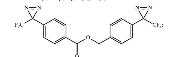
4-(3-(trifluoromethyl)-3H-diazirin-3-yl)benzyl 4-(3-(trifluoromethyl)-3H-diazirin-3-yl)benzoate
