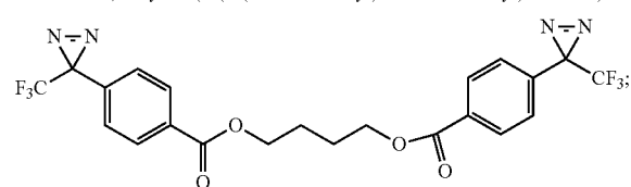
butane-1,4-diyl bis(4-(3-(trifluoromethyl)-3H-diazirin-3-yl)benzoate)
