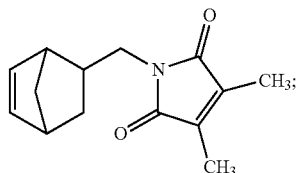
1-(bicyclo[2.2.1]hept-5-en-2-ylmethyl)-3,4-dimethyl-1H-pyrrole-2,5-dione (MeDMMINB)
