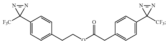
4-(3-(trifluoromethyl)-3H-diazirin-3-yl)phenethyl 2-(4-(3-(trifluoromethyl)-3H-diazirin-3-yl)phenyl)acetate
