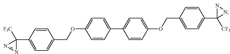
4,4'-bis((4-(3-(trifluoromethyl)-3H-diazirin-3-yl)benzyl)oxy)-1,1'-biphenyl
