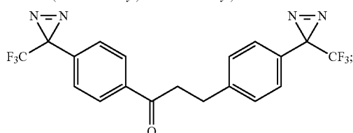
1,3-bis(4-(3-(trifluoromethyl)-3H-diazirin-3-yl)phenyl)propan-1-one
