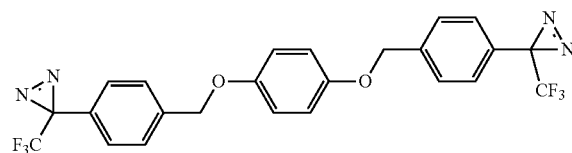
1,4-bis(4-(3-(trifluoromethyl)-3H-diazirin-3-yl)benzyl)oxy)benzene
