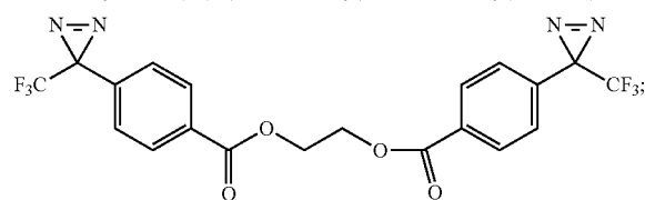
ethane-1,2-diyl bis(4-(3-(trifluoromethyl)-3H-diazirin-3-yl)benzoate)
