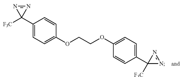
1,2-bis(4-(3-(trifluoromethyl)-3H-diazirin-3-yl)phenoxy)ethane
