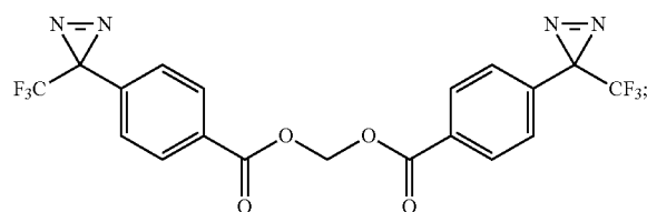
methylene bis(4-(3-(trifluoromethyl)-3H-diazirin-3-yl)benzoate)
