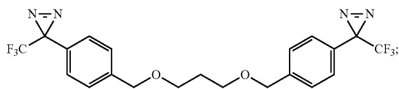
1,3-bis((4-(3-(trifluoromethyl)-3H-diazirin-3-yl)benzyl)oxy)propane
