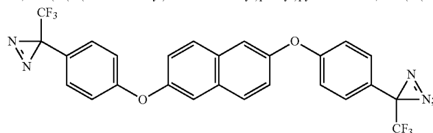
2,6-bis(4-(3-(trifluoromethyl)-3H-diazirin-3-yl)phenoxy)naphthalene
