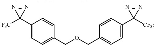
3,3'-((oxybis(methylene))bis(4,1-phenylene))bis(3-(trifluoromethyl)-3H-diazirine)
