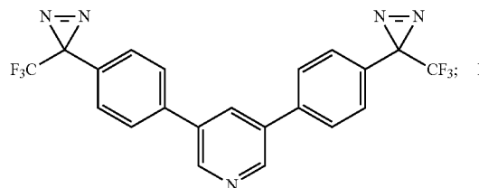
3,5-bis(4-(3-(trifluoromethyl)-3H-diazirin-3-yl)phenyl)pyridine
