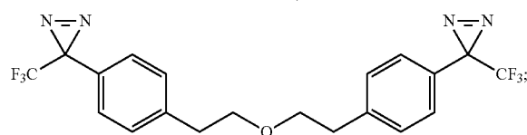
3,3'-((oxybis(ethane-2,1-diyl))bis(4,1-phenylene))bis(3-(trifluoromethyl)-3H-diazirine)
