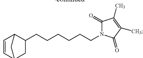
1-(6-(bicyclo[2.2.1]hept-5-en-2-yl)hexyl)-3,4-dimethyl-1H-pyrrole-2,5-dione (HexDMMINB)
