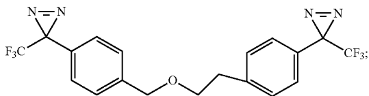
3-(trifluoromethyl)-3-((4-(2-((4-(3-(trifluoromethyl)-3H-diazirin-3-yl)benzyl)oxy)ethyl)phenyl)-3H-diazirine
