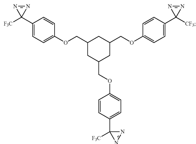
1,3,5-tris((4-(3-(trifluoromethyl)-3H-diazirin-3-yl)phenoxy)methyl)cyclohexane
