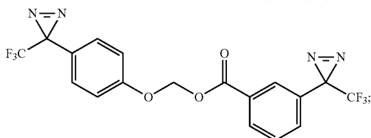
(4-(3-(trifluoromethyl)-3H-diazirin-3-yl)phenoxy)methyl 3-(3-(trifluoromethyl)-3H-diazirin-3-yl)benzoate
