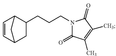
1-(3-(bicyclo[2.2.1]hept-5-en-2-yl)propyl)-3,4-dimethyl-1H-pyrrole-2,5-dione (PrDMMINB)
