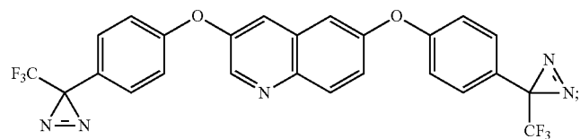
3,6-bis(4-(3-(trifluoromethyl)-3H-diazirin-3-yl)phenoxy)quinoline
