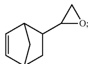
2-(bicyclo[2.2.1]hept-5-en-2-yl)oxirane
