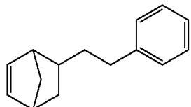
5-phenethylbicyclo[2.2.1]hept-2-ene (PENB)
