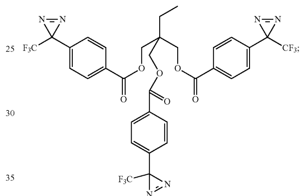
2-ethyl-2-(((4-(3-(trifluoromethyl)-3H-diazirin-3-yl)benzoyl)oxy)methyl)propane-1,3-diyl bis(4-(3-(trifluoromethyl)-3H-diazirin-3-yl)benzoate)
