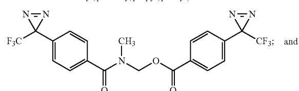
(N-methyl-4-(3-(trifluoromethyl)-3H-diazirin-3-yl)benzamido)methyl 4-(3-(trifluoromethyl)-3H-diazirin-3-yl)benzoate
