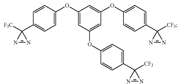
1,3,5-tris(4-(3-(trifluoromethyl)-3H-diazirin-3-yl)phenoxy)benzene
