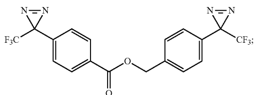
4-(3-(trifluoromethyl)-3H-diazirin-3-yl)benzyl 4-(3-(trifluoromethyl)-3H-diazirin-3-yl)benzoate
