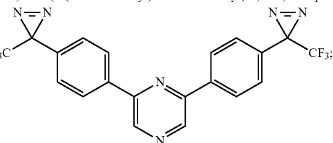
2,6-bis(4-(3-(trifluoromethyl)-3H-diazirin-3-yl)phenyl)pyrazine
