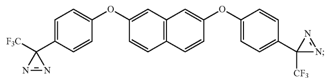
2,7-bis(4-(3-(trifluoromethyl)-3H-diazirin-3-yl)phenoxy)naphthalene
