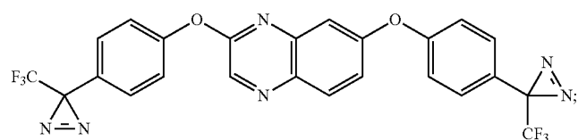
2,7-bis(4-(3-(trifluoromethyl)-3H-diazirin-3-yl)phenoxy)quinoxaline
