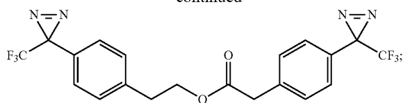
4-(3-(trifluoromethyl)-3H-diazirin-3-yl)phenethyl 2-(4-(3-(trifluoromethyl)-3H-diazirin-3-yl)phenyl)acetate
