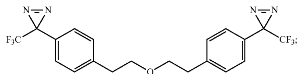
3,3'-((oxybis(ethane-2,1-diyl))bis(4,1-phenylene))bis(3-(trifluoromethyl)-3H-diazirine)
