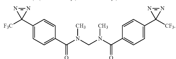
N,N'-methylenebis(N-methyl-4-(3-(trifluoromethyl)-3H-diazirin-3-yl)benzamide)
