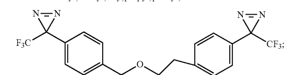
3-(trifluoromethyl)-3-(4-(2-((4-(3-(trifluoromethyl)-3H-diazirin-3-yl)benzyl)oxy)ethyl)phenyl)-3H-diazirine
