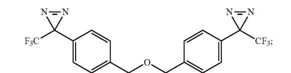
3,3'-((oxybis(methylene))bis(4,1-phenylene))bis(3-(trifluoromethyl)-3H-diazirine)
