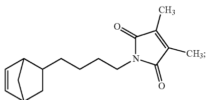
1-(4-(bicyclo[2.2.1]hept-5-en-2-yl)butyl)-3,4-dimethyl-1H-pyrrole-2,5-dione (BuDMMINB)
