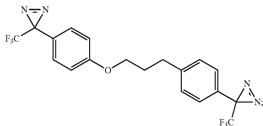
3-(trifluoromethyl)-3-((4-(3-(4-(3-(trifluoromethyl)-3H-diazirin-3-yl)phenoxy)propyl)phenyl)-3H-diazirine
