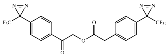
2-oxo-2-(4-(3-(trifluoromethyl)-3H-diazirin-3-yl)phenyl)ethyl 3-(3-(trifluoromethyl)-3H-diazirin-3-yl)benzoate
