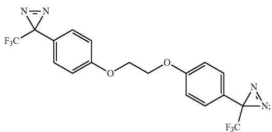
1,2-bis(4-(3-(trifluoromethyl)-3H-diazirin-3-yl)phenoxy)ethane
