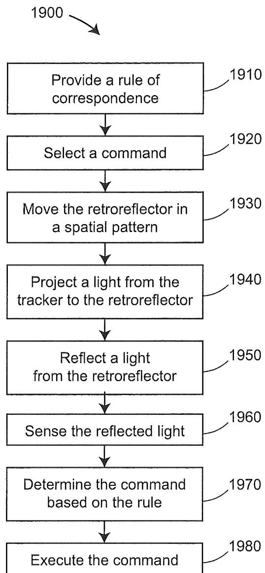
FIGURE 19
