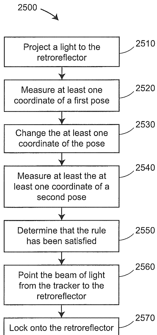
FIGURE 25
