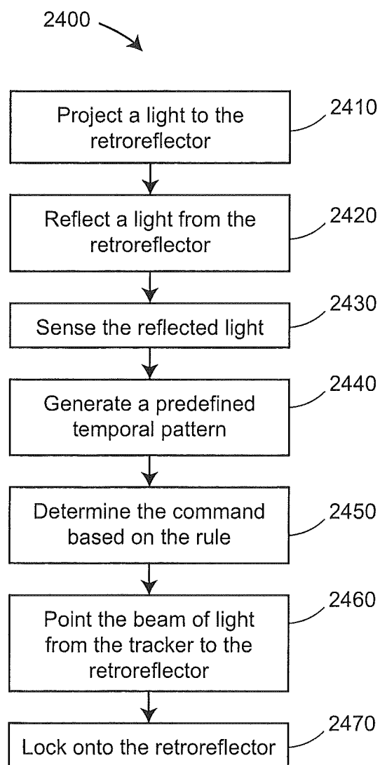
FIGURE 24
