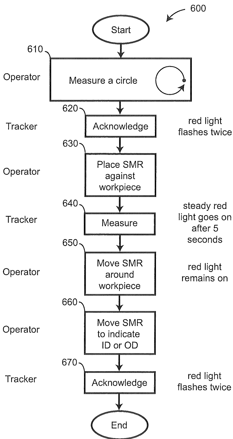
FIGURE 15
