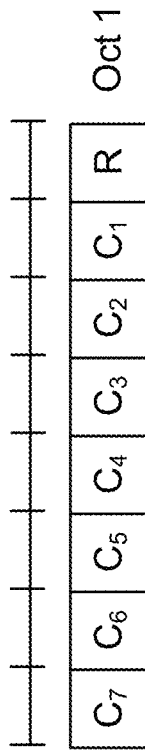
A) Activation/Deactivation MAC Control Element with one oct
