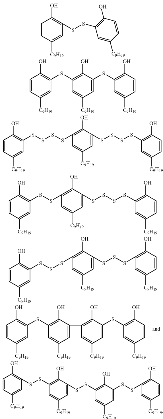
Photoconductive Layer Components
