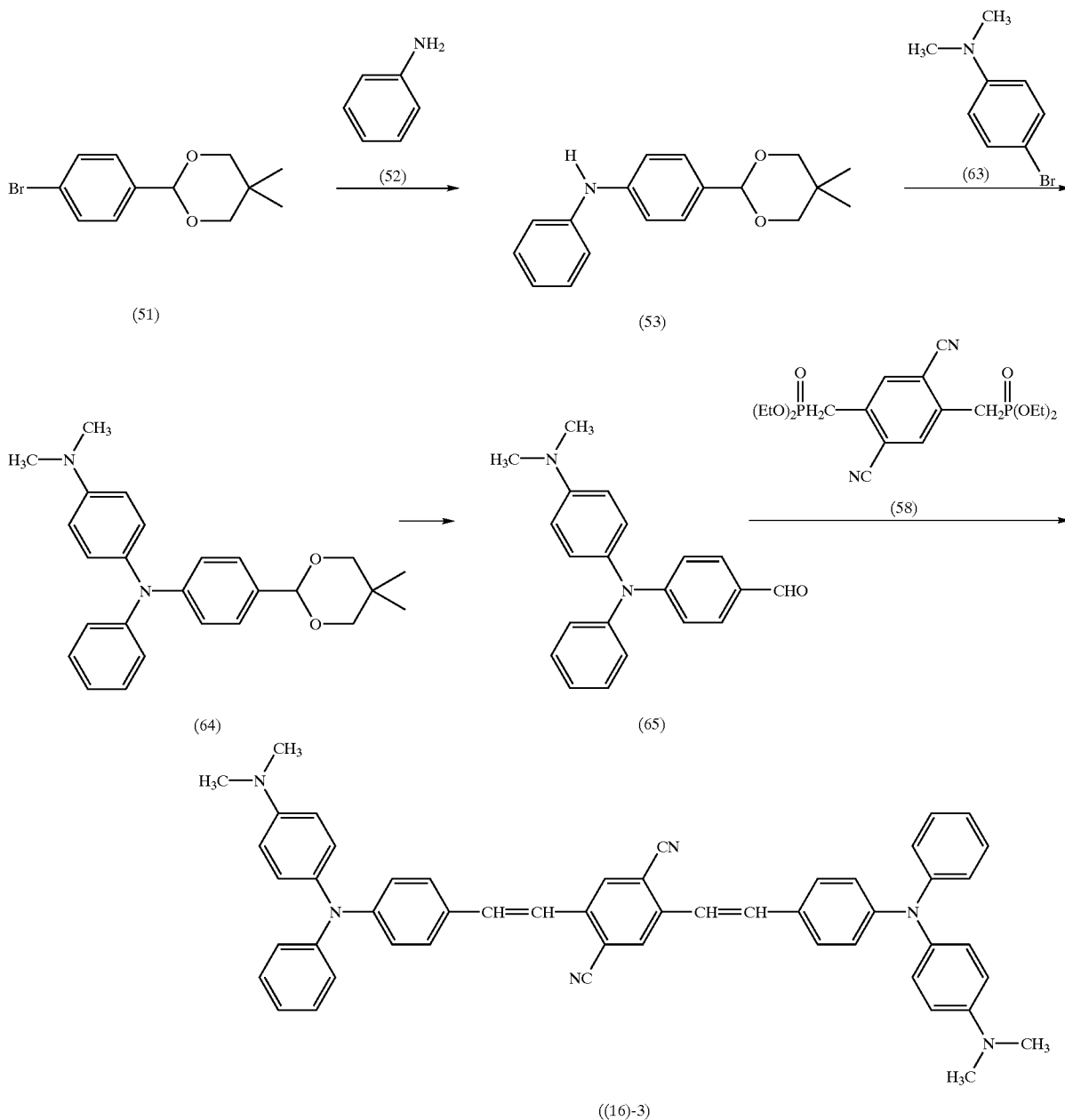
Reaction scheme 6
