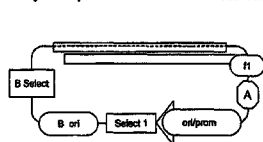
Eukaryotic expression vector basis for cassette(s) of (A)
