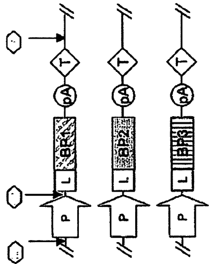
Eukaryotic expression cassettes for different binding proteins
