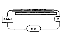
Prokaryotic expression vector basis for cassette(s) of (A)
