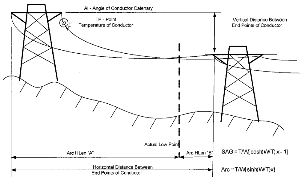
Catenary Curve for Wire Conductor suspend from towers
