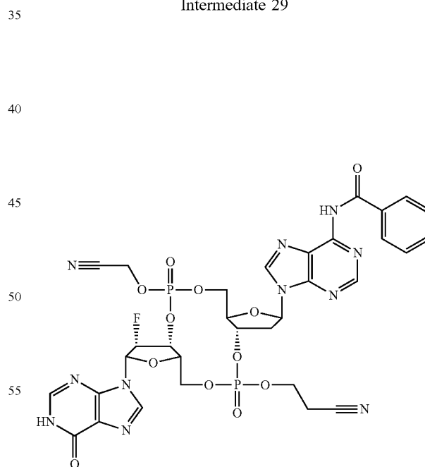
(3',3')Cyclic-[3'-O(CE)phosphotriester-N 6 (Bz)-2'-deoxyAdenosine]-[3'-O(CE)phosphotriester-2'-deoxy-2'-fluoroInosine]
