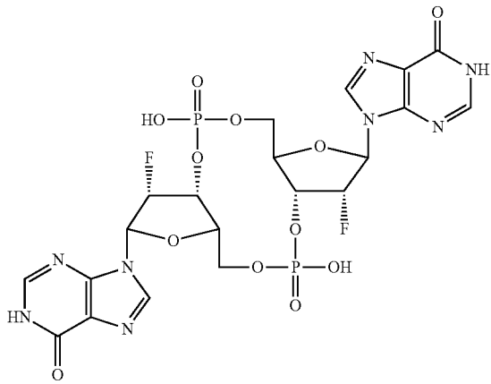
c-di(2'FdIMP)
