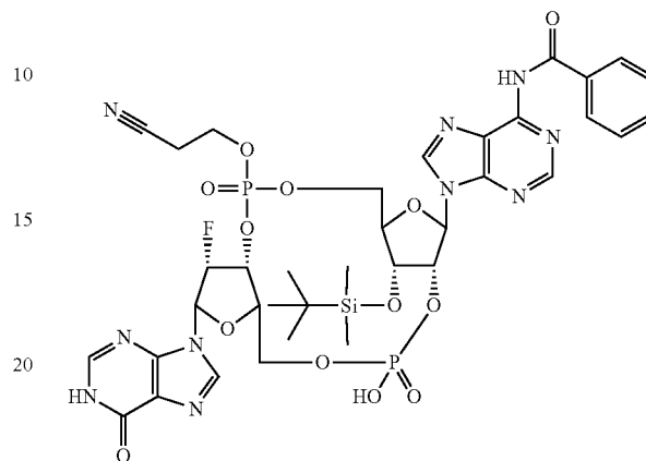
Cyclic-(2',3')-[2'-O-(CE)phosphotriester-3'-O-TBDMS-N 6 (Bz)Adenosine]-[3'-O-(CE)phosphotriester-2'-deoxy-2'-fluorinosine]
