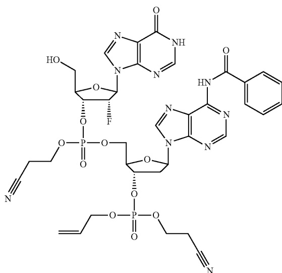
[3'-O(CE)phosphotriester-2'-deoxy-2'-fluoroInosine]-(3',5')-[3'-O(Allyl,CE)phosphotriester-N 6 (Bz)-2'-deoxyAdenosine]
