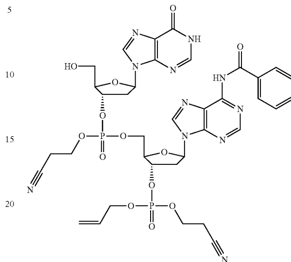
[3'-O(CE)phosphotriester-2'-deoxyInosine]-(3',5')-[3'-O(Allyl,CE)phosphotriester-N 6 (Bz)-2'-deoxyAdenosine]
