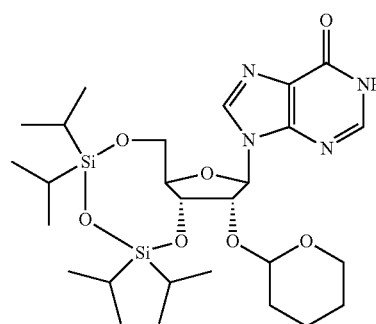
(5',3')-O(TIPS)-2'-O(Thp)Inosine
