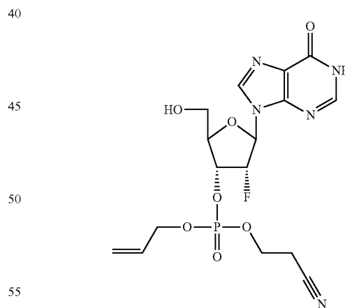
3'-O-(Allyl, CE)phosphotriester-2'-deoxy-2'-fluorinosine
