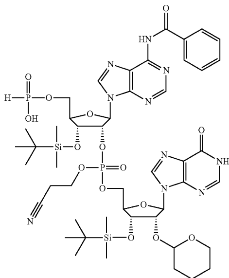
[5'-O(H-phosphonate)-3'-O(TBDMS)-2'-O(CE)phosphotriester-N 6 (Bz)Adenosine]-(3',5')-[3'-O(TBDMS)-2'-O(Thp)Inosine]
