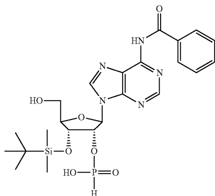
3'-O(TBDMS)-2'-O(H-phosphonate)-N 6 (Bz)Adenosine
