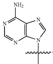
Adenine
