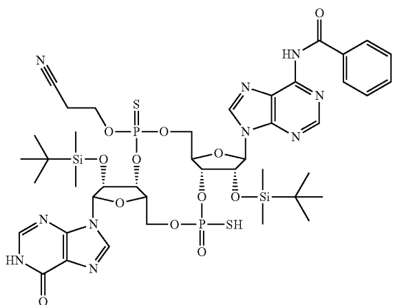
(3',3')Cyclic-[2'-O(TBDMS)-3'-O(phosphorothioate-diester)-N 6 (Bz)Adenosine]-[2'-O(TBDMS)-3'-O(CE)phosphorothioate-triester-Inosine]
