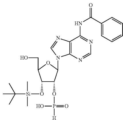
2'-O-(H-phosphonate)-3'-O-TBDMS-N 6 (Bz)-Adenosine
