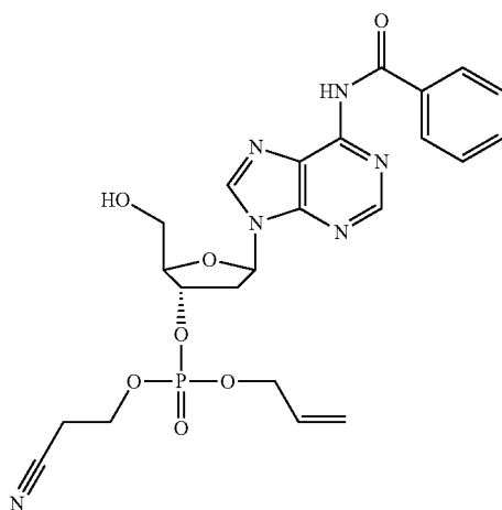
3'-O[(Allyl,CE)phosphotriester]-N 6 (Bz)-2'-deoxyAdenosine
