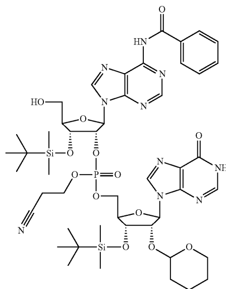
[3'-O(TBDMS)-2'-O(CE)phosphotriester-N 6 (Bz)Adenosine]-(3',5')-[3'-O(TBDMS)-2'-O(Thp)Inosine]
