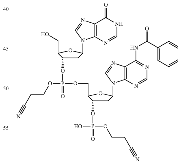
[3'-O(CE)phosphotriester-2'-deoxyInosine]-(3',5')-[3'-O(CE)phosphodiester-N 6 (Bz)-2'-deoxyAdenosine]
