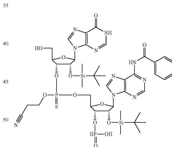
[2'-O(TBDMS)-3'-O(CE)phosphorothioate-triester-Inosine]-(3',5')-[2'-O(TBDMS)-3'-O(H-phosphonate)-N 6 (Bz)Adenosine]
