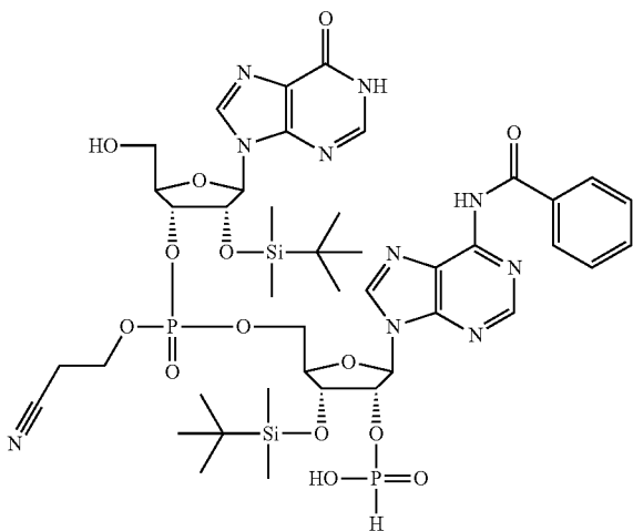
[2'-O(TBDMS)-3'-O(CE)phosphotriester-Inosine]-(3',5')-[3'-O(TBDMS)-2'-O(H-phosphonate)-N 6 (Bz)Adenosine]
