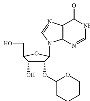
2'-O(Thp)Inosine
