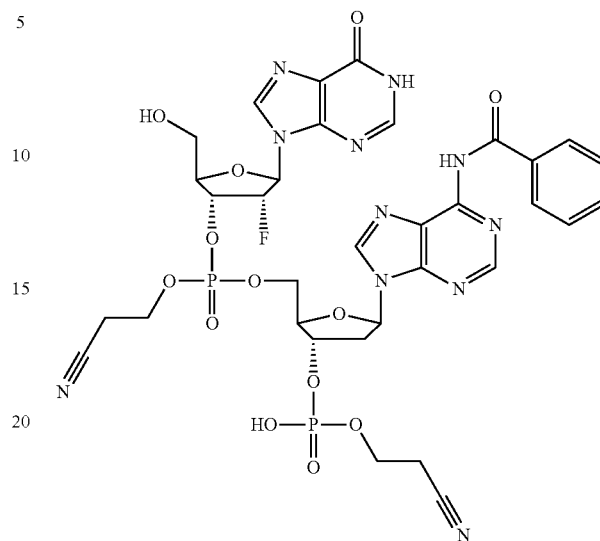
[3'-O(CE)phosphotriester-2'-deoxy-2'-fluoroInosine]-(3',5')-[3'-O(CE)phosphodiester-N 6 (Bz)-2'-deoxyAdenosine]
