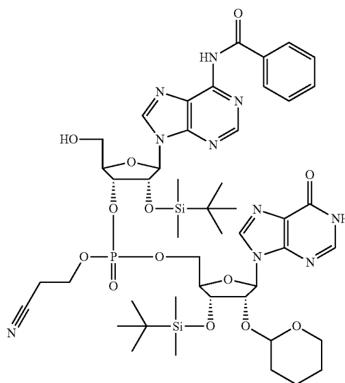
[2'-O(TBDMS)-3'-O(CE)phosphotriester-N 6 (Bz)Adenosine]-(3',5')-[3'-O(TBDMS)-2'-O(Thp)inosine]
