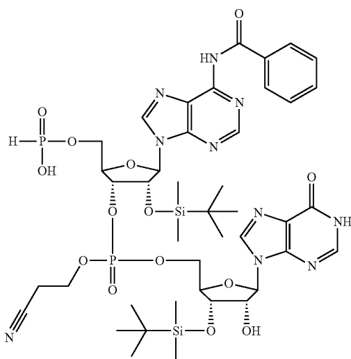
[5'-O(H-phosphonate)-2'-O(TBDMS)-3'-O(CE)phosphotriester-N 6 (Bz)Adenosine]-(3',5')-[3'-O(TBDMS)Inosine]
