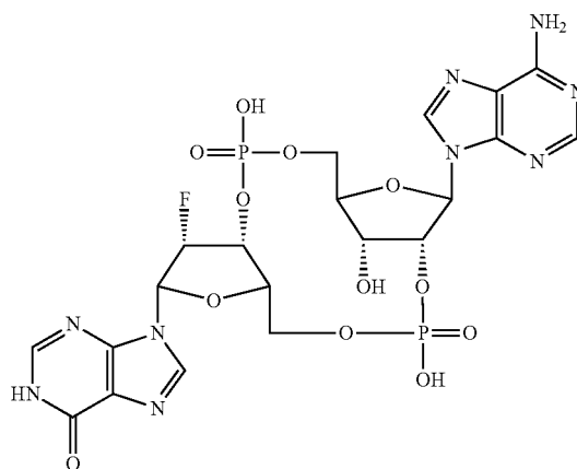
(2',3')c-(AMP-2'FdIMP)
