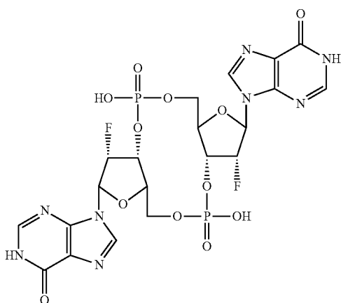
c-di(2'FdIMP)
