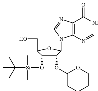
3'-O(TBDMS)-2'-O(Thp)inosine
