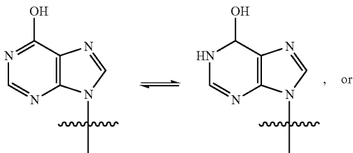
Hypoxanthine
