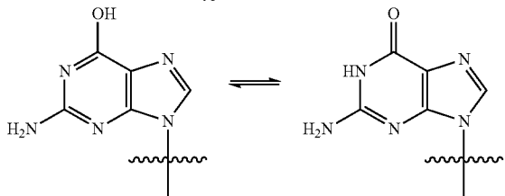
Guanine
