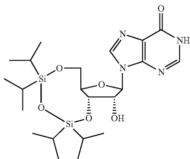
(5',3')-O(TIPS)Inosine
