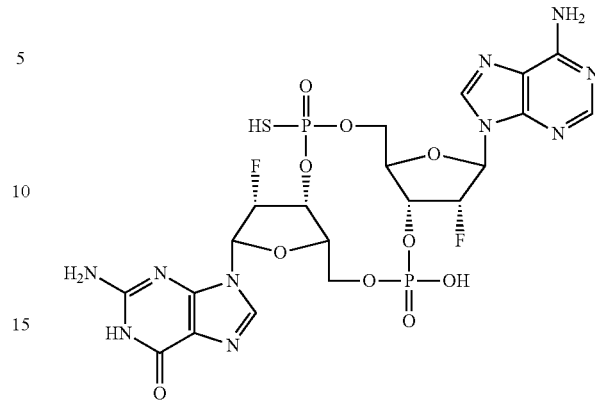
c-[2'FdGMP(S)-2'FdAMP(S)]
