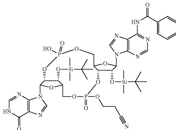
(3',2')Cyclic-[2'-O(TBDMS)-3'-O(CE)phosphotriester-N 6 (Bz)Adenosine]-[2'-O(phosphodiester)-3'-O(TBDMS)Inosine]
