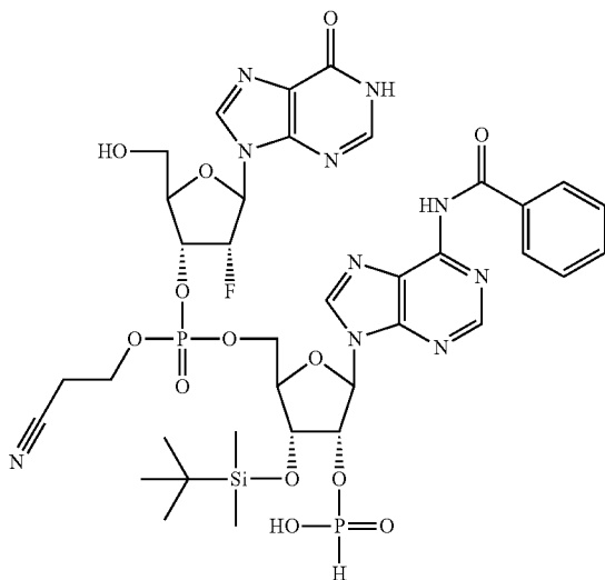
[3'-O-(CE)phosphotriester-2'-deoxy-2'-fluorinosine]-(3',5')-[2'-O-(H-phosphonate)-3'-O-TBDMS-N 6 (Bz)-Adenosine]
