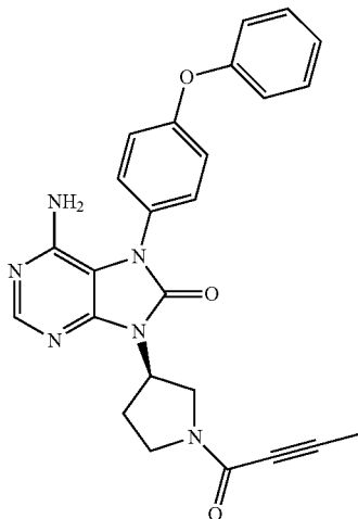
[Chemical Formula 4]
