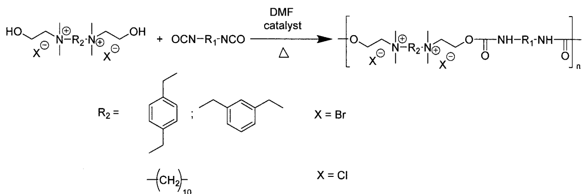
Scheme 5. Preparation of homo polyurethanes from diol monomers bearing two quaternary ammonium salts
