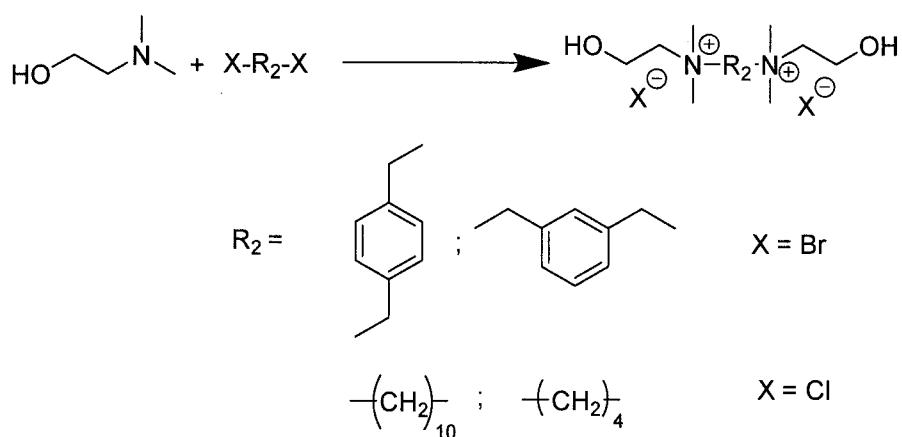
Scheme 4. Preparation of diol monomers bearing two quaternary ammonium salts
