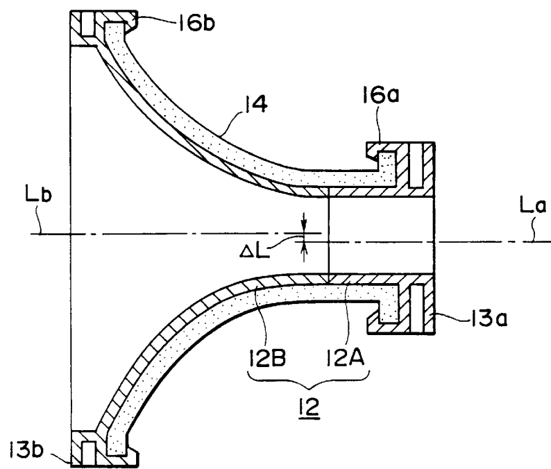
FIG. 13 (PRIOR ART)
