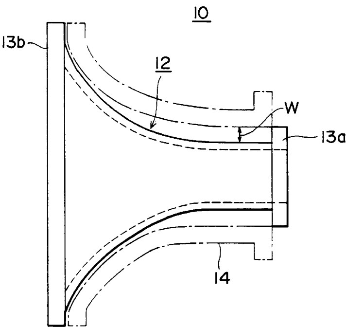
FIG. 13 (PRIOR ART)
