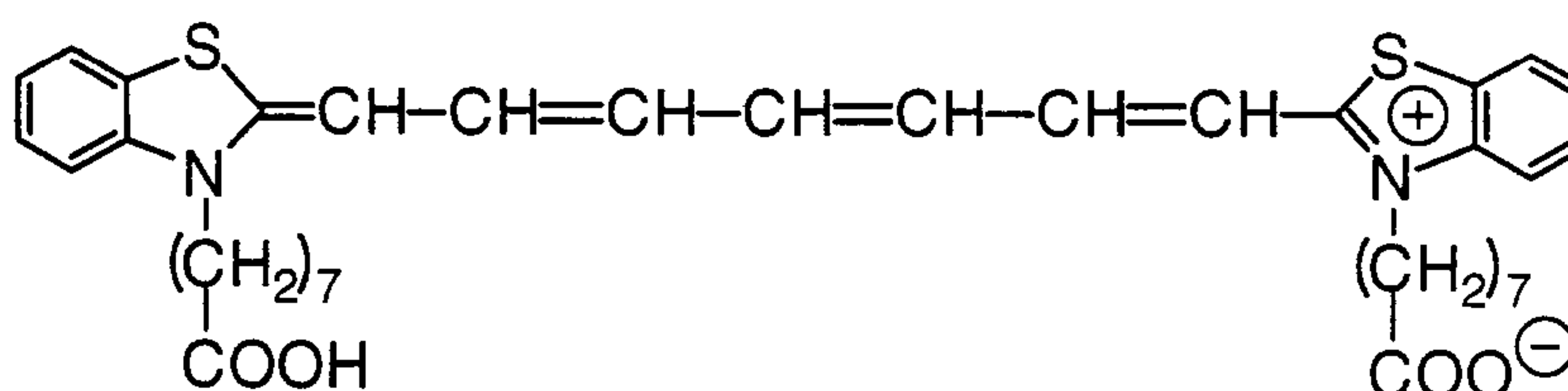
Disulfide compound A
