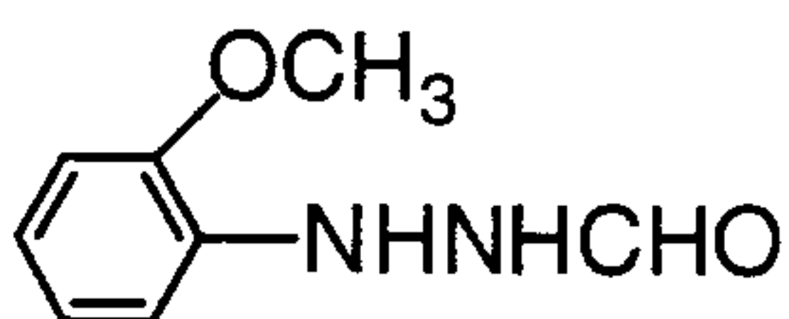
Hydrazine derivative H-62u
