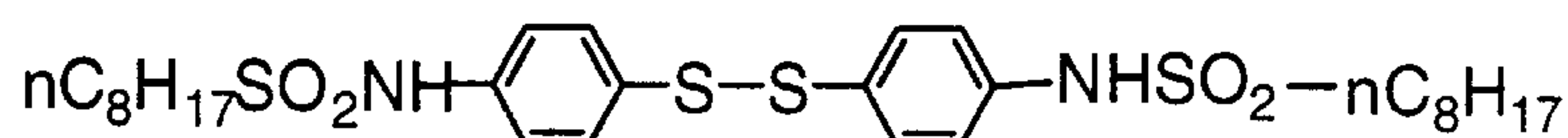
Disulfide compound A
