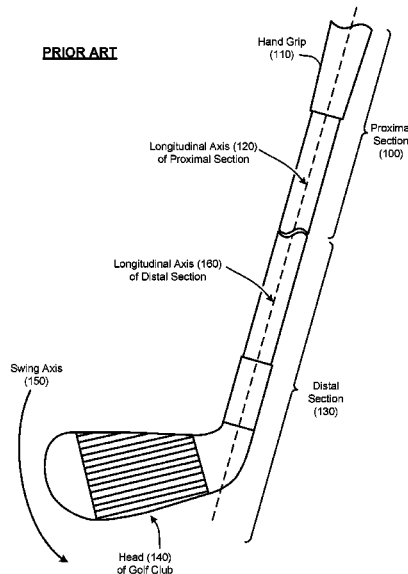
Typical Prior Art Golf Club
