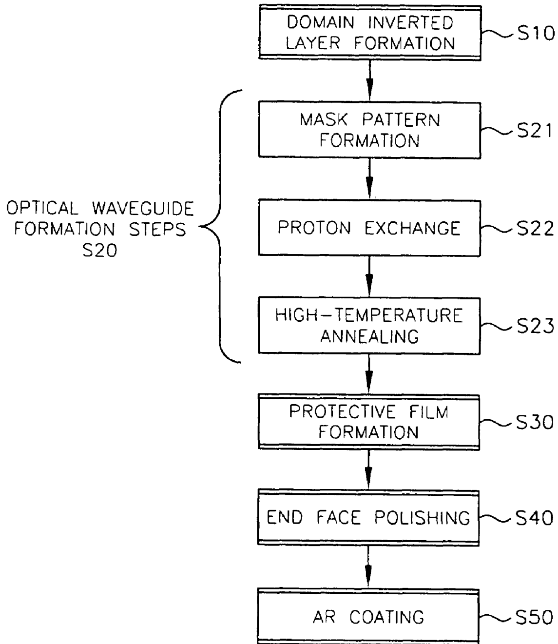
FIG. 3 (Prior Art)
