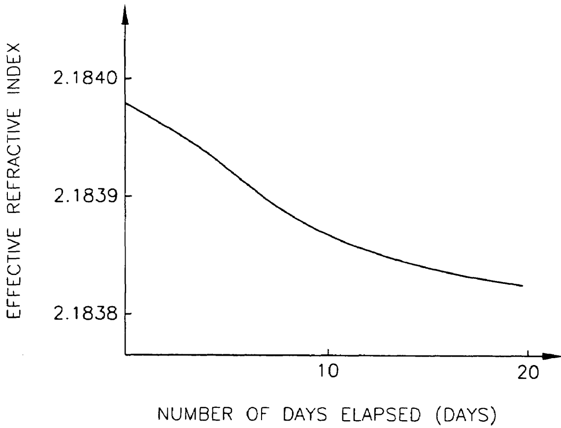
FIG. 6 (Prior Art)
