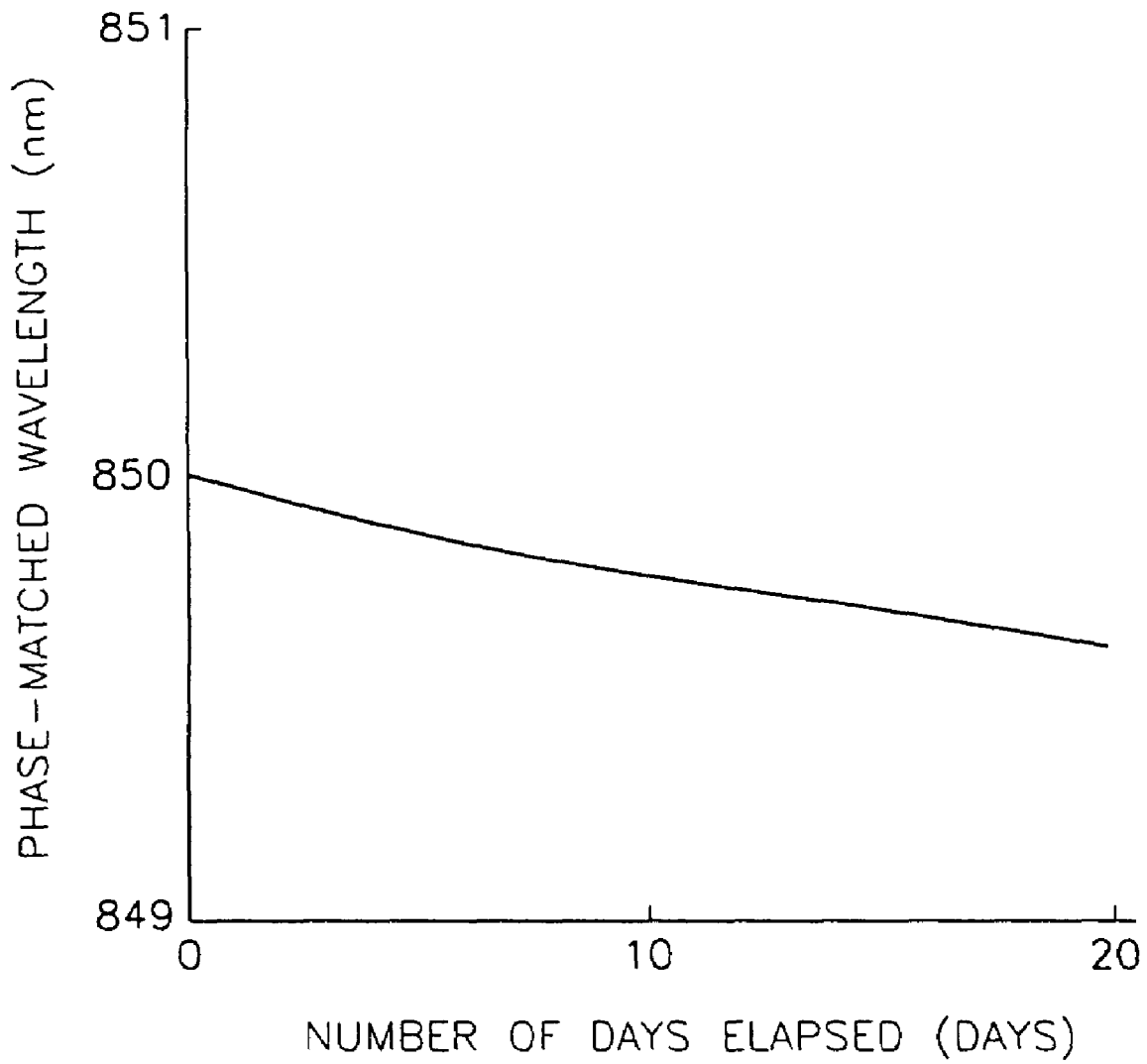
FIG. 5 (Prior Art)
