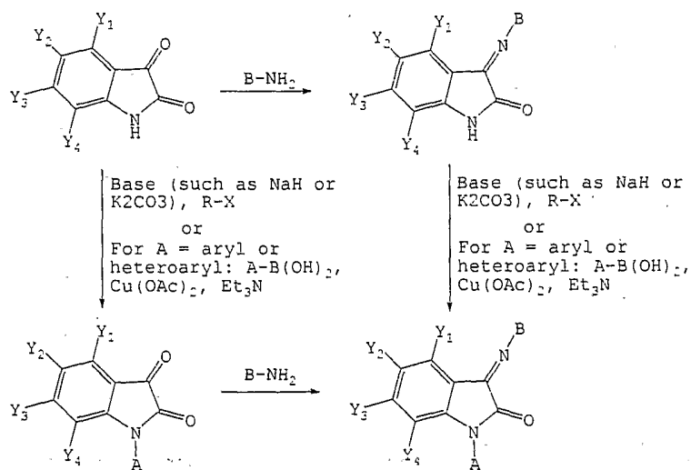
Scheme 9 a . Synthesis of Substituted Iminoindolones
