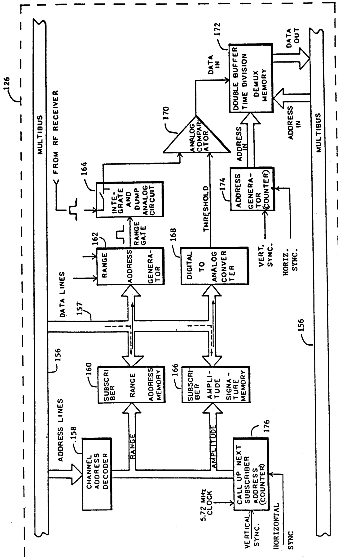
FIG. 16 DIGITAL INTERFACE FOR RADIO CENTRAL OFFICE
