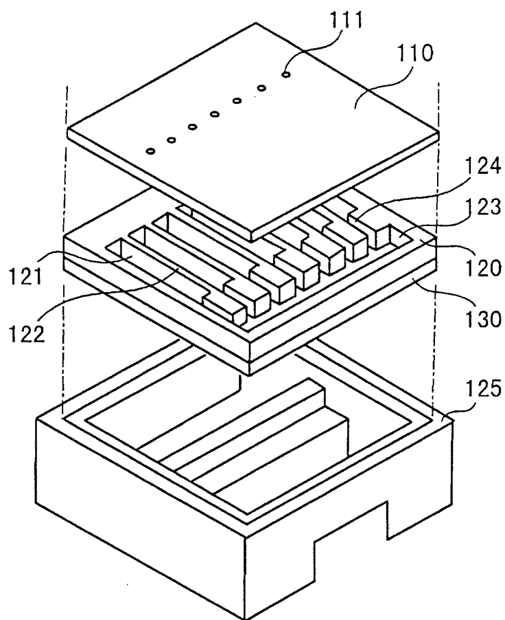
1a: INK JET HEAD
