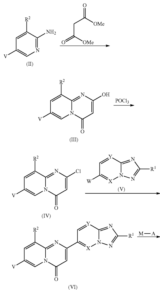
Scheme 1. General preparation of compounds of formula (I).
