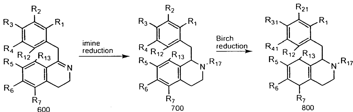
Reaction Scheme 1
