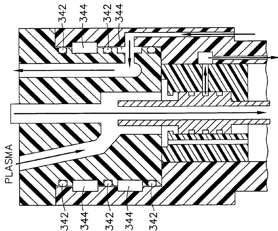
FIG. 33a (COOLING FLUID PASSAGEWAYS)
