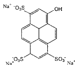
(the Na^+ salt of HPTS—"pyranine")
