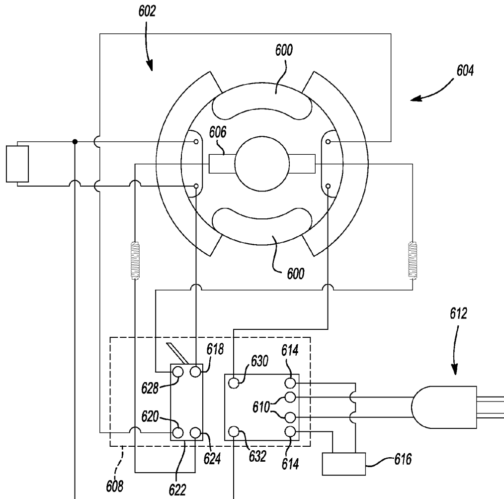
Fig-6 PRIOR ART
