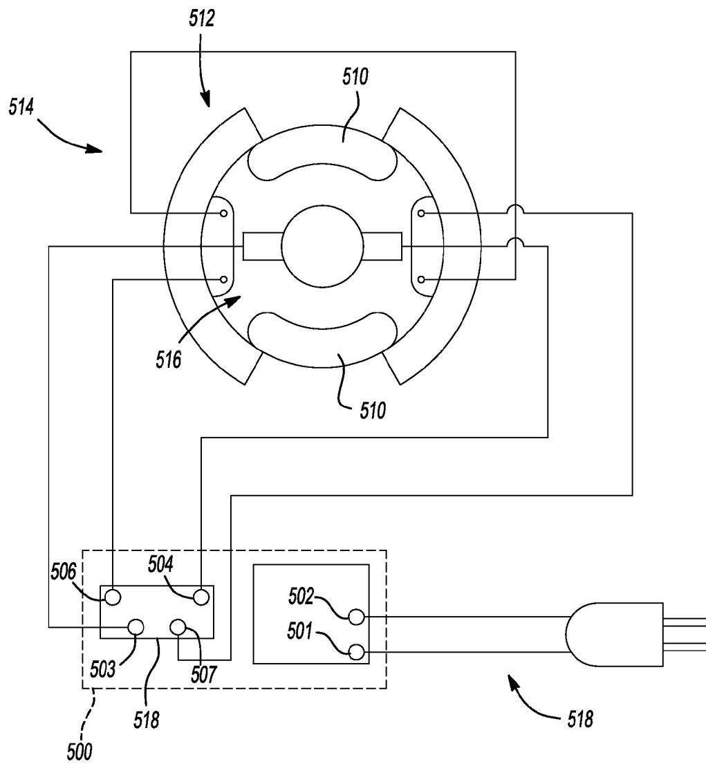
Fig-5 PRIOR ART
