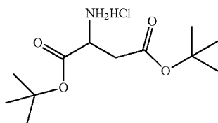
L-aspartic acid di-t-butyl ester hydrochloride
