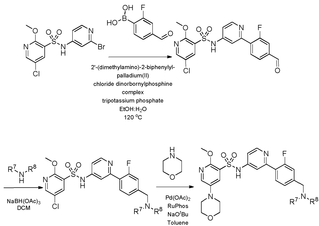
Scheme 5
