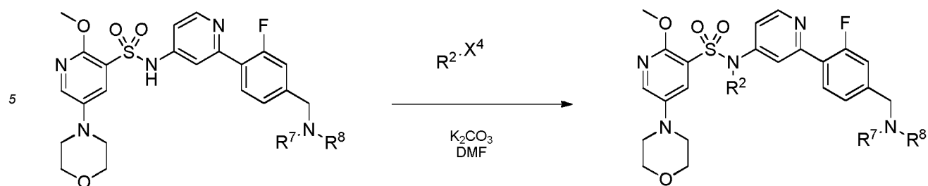
Scheme 9
