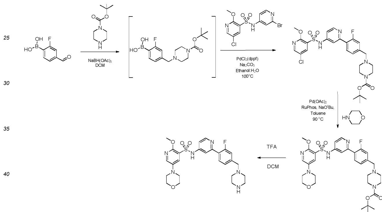
Scheme 10
