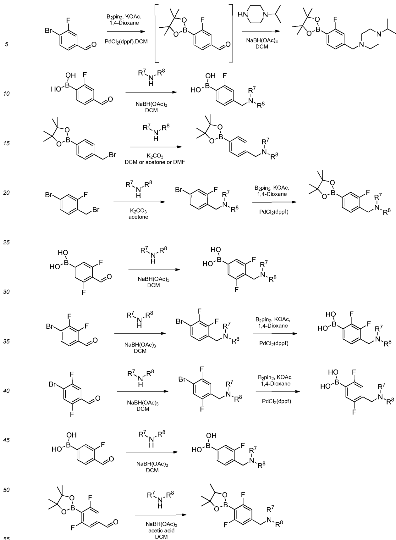
Scheme 1
