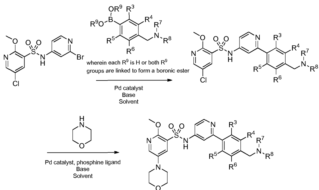
Scheme 4
