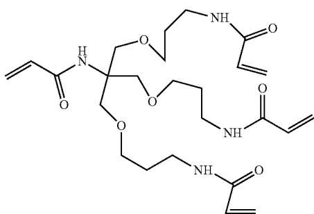
Structural Formula 1
