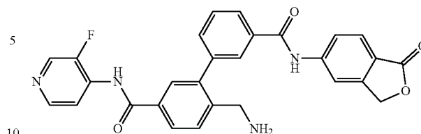
Compound 11
