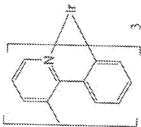
HILx Iridium(III)tris(3- methyl-2-phenylpyridine)
