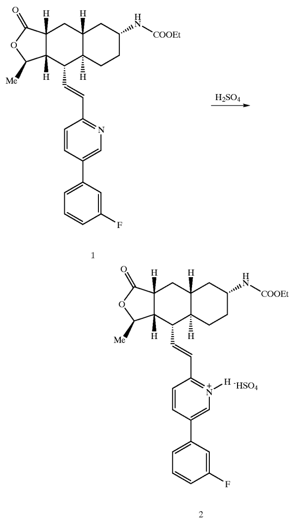
Scheme I: General Synthesis of Compound 2
