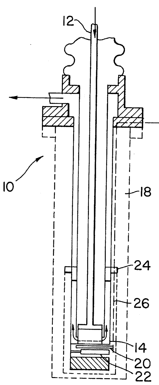
FIG. 1 (PRIOR ART)
