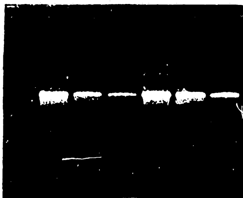
Figure 3. KlenTaq1 is more thermostable than AmpliTaq.
