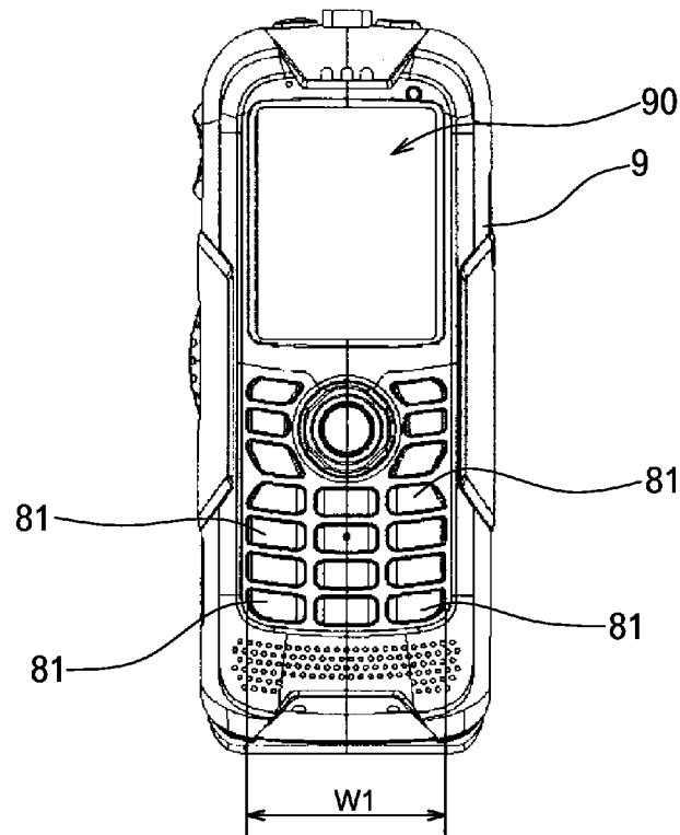
FIG. 6 PRIOR ART
