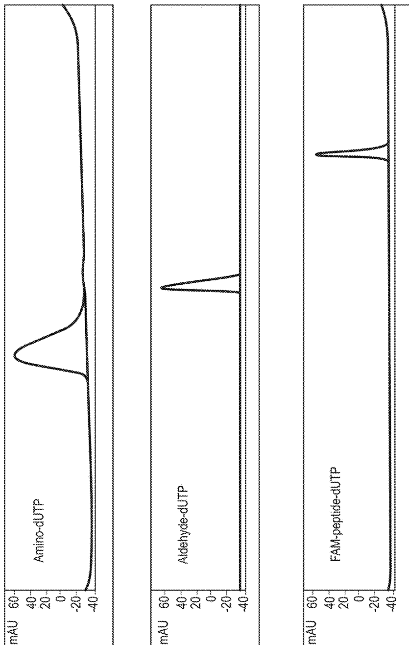
HPLC Analysis of Modified dUTPs
