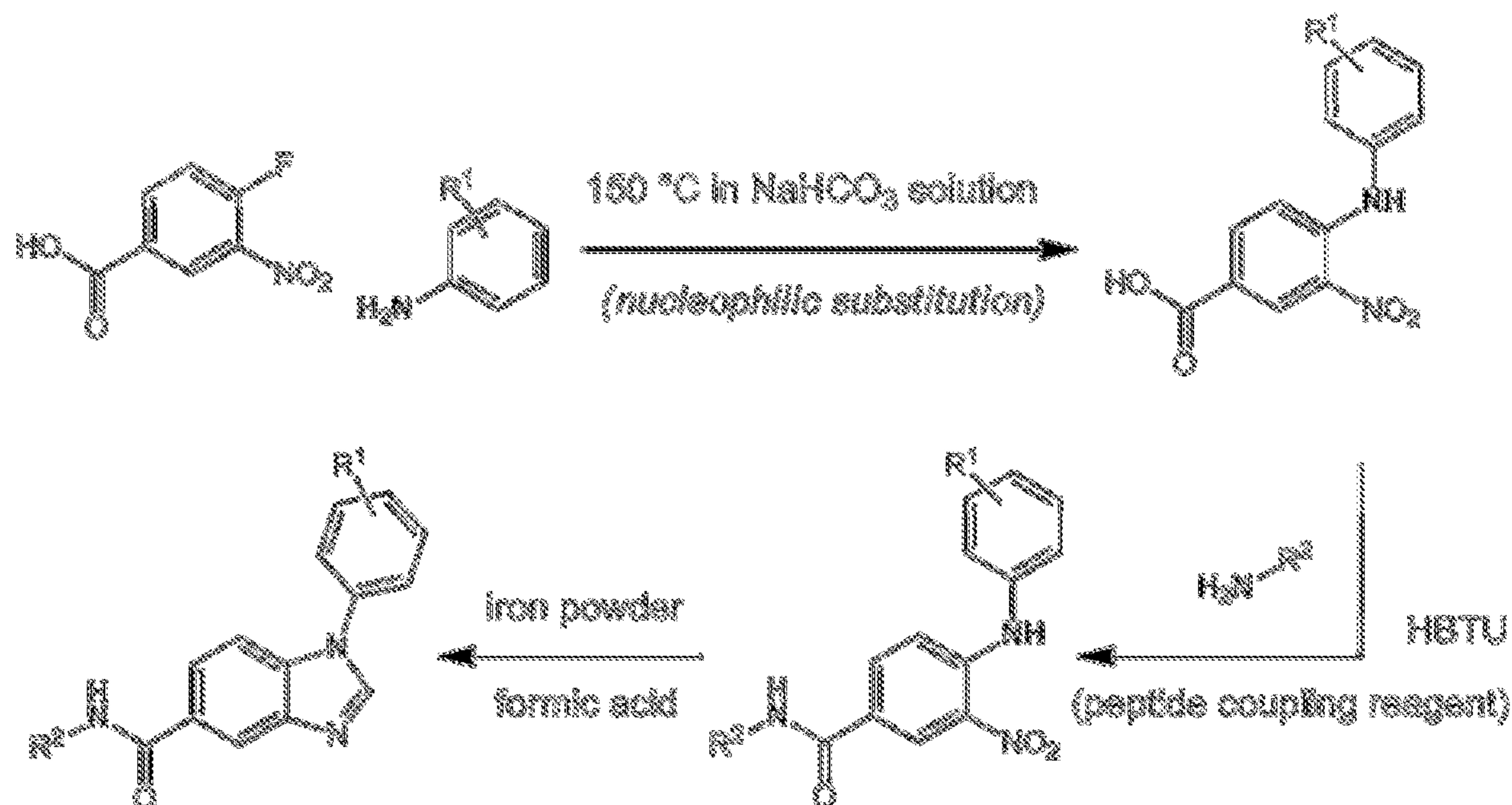
Scheme 1. Exemplary synthesis of compounds of Formula (I).
