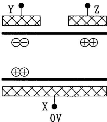
FIG. 5C Related Art
