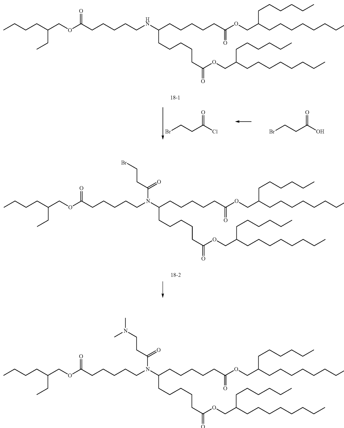
Compound I-36
