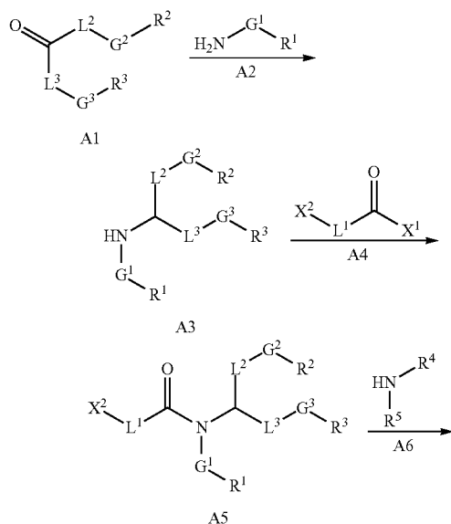
GENERAL REACTION SCHEME 1
