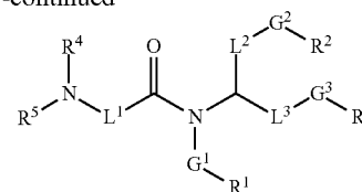
Compound I
