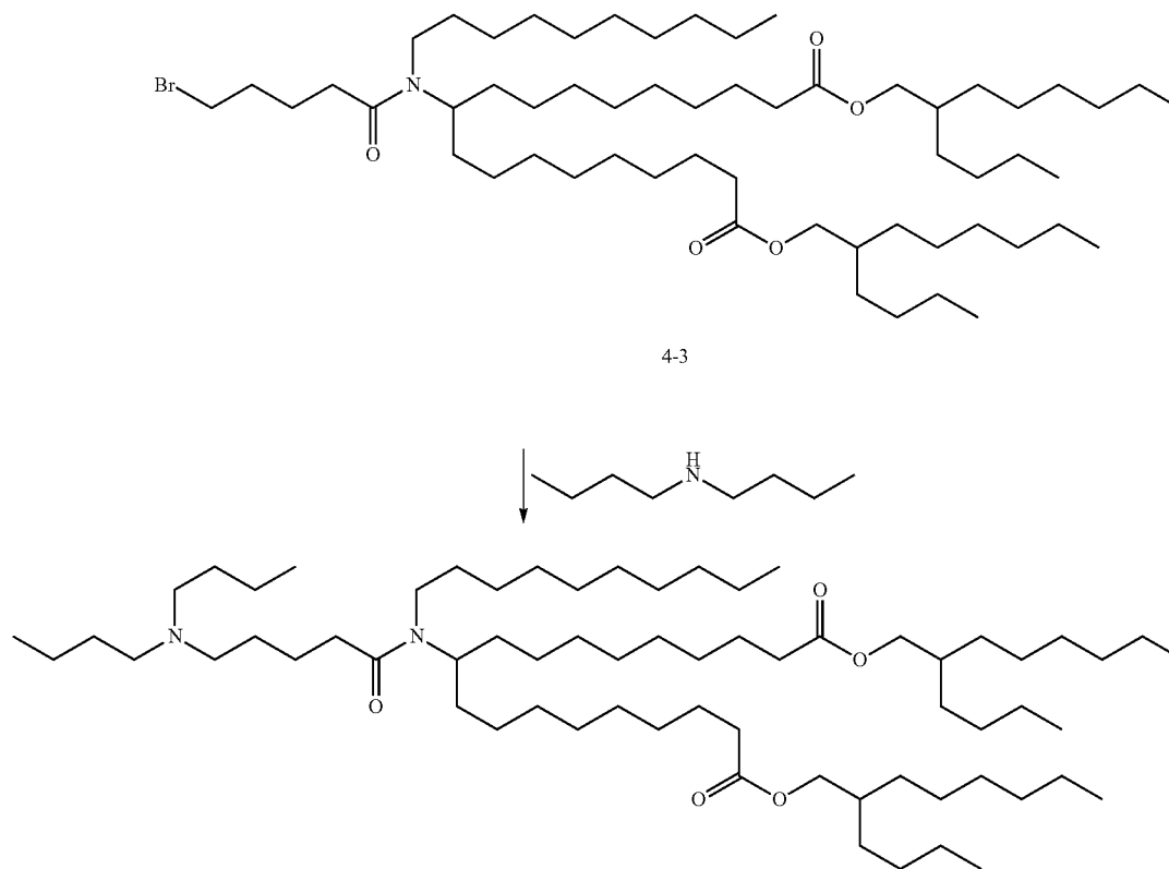
Compound I-31
