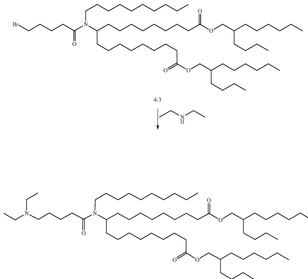
Compound I-8
