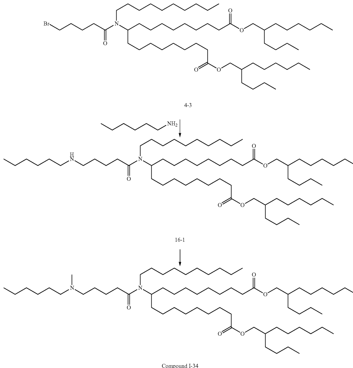
Compound I-34
