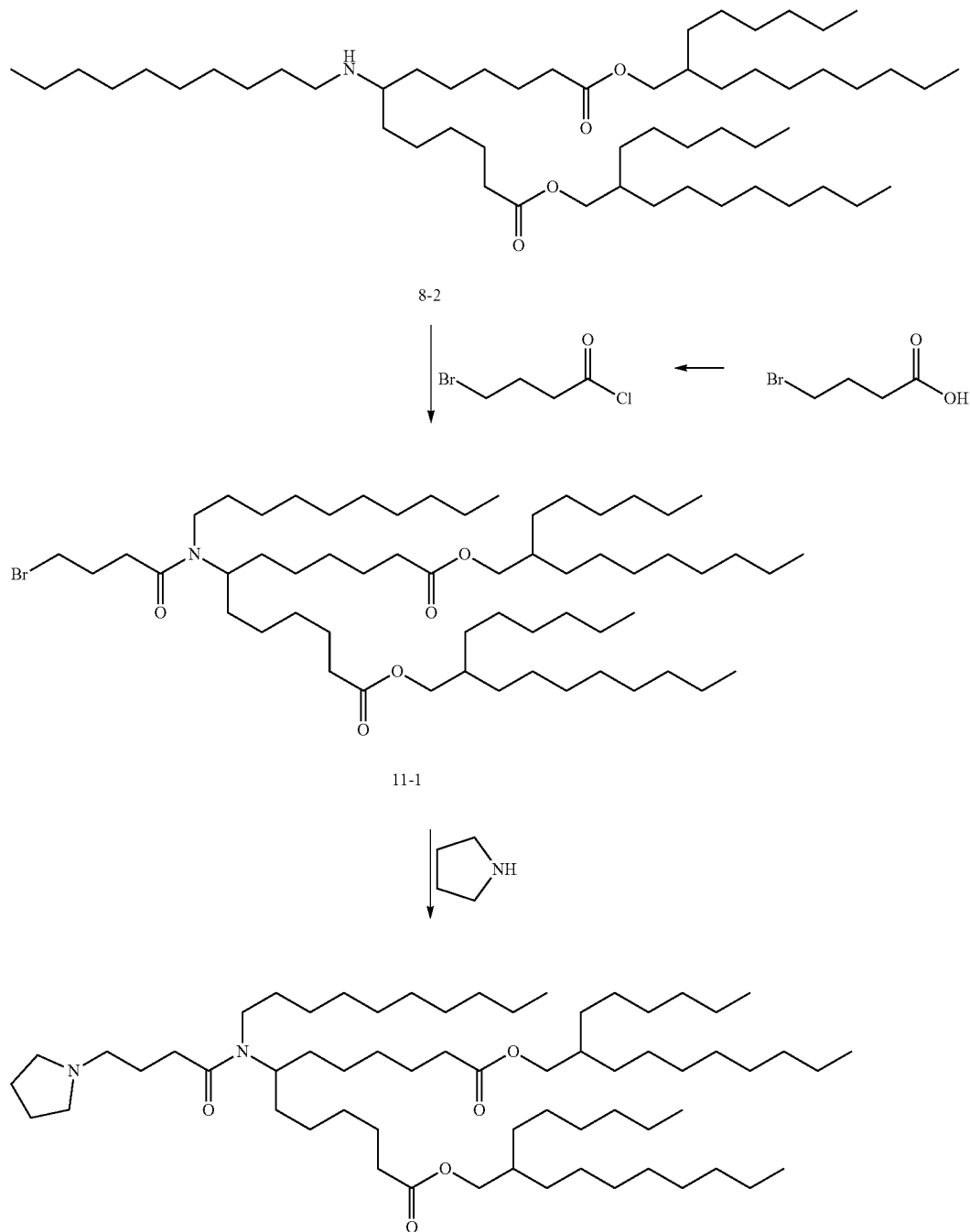
Compound I-29
