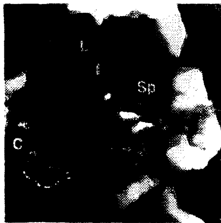
BJ66lux Infection (7 d p.i.)
