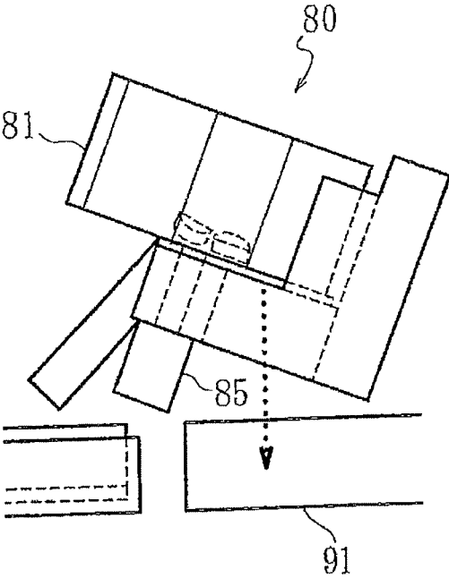
FIG.13 (c)
