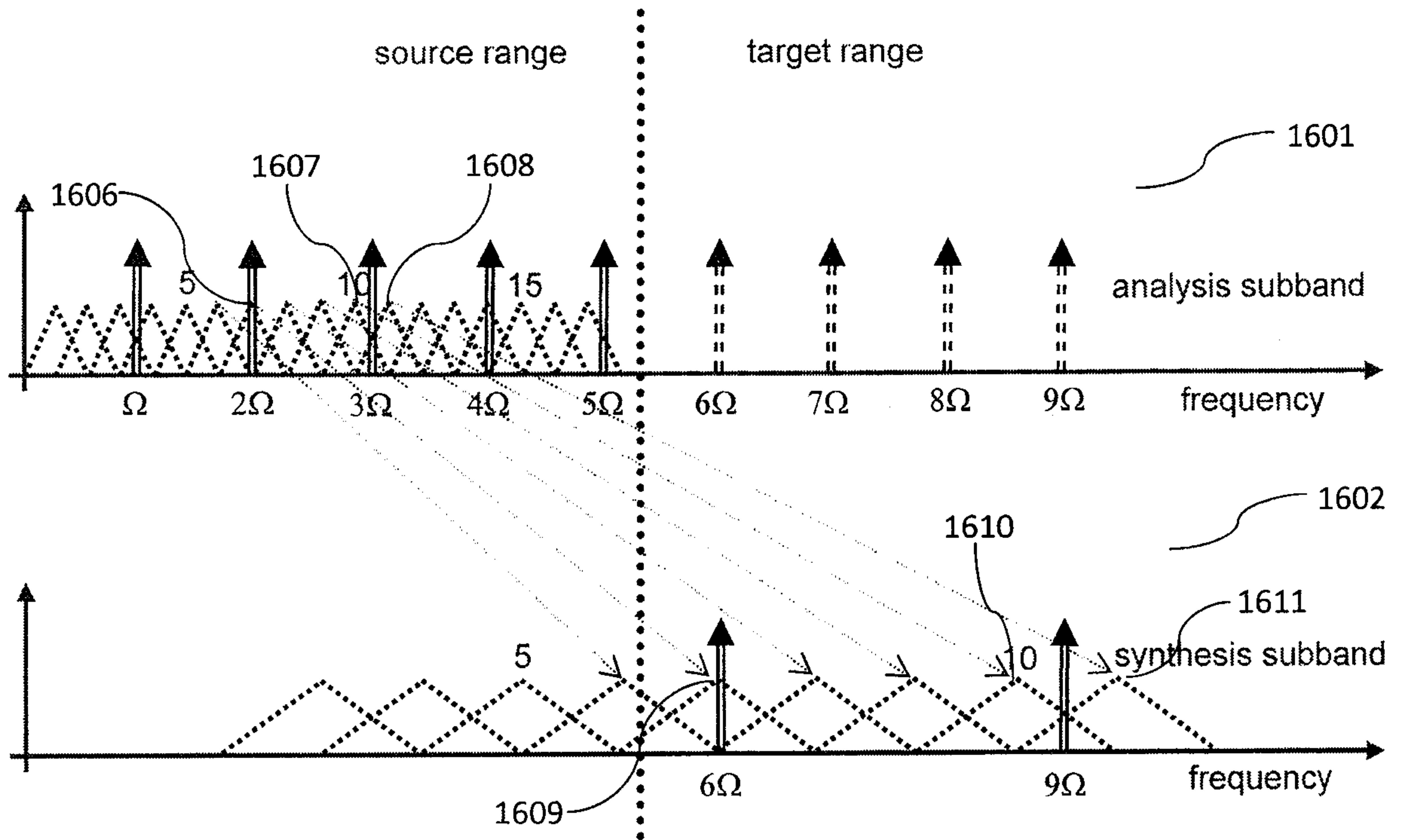
Fig. 16 - PRIOR ART
