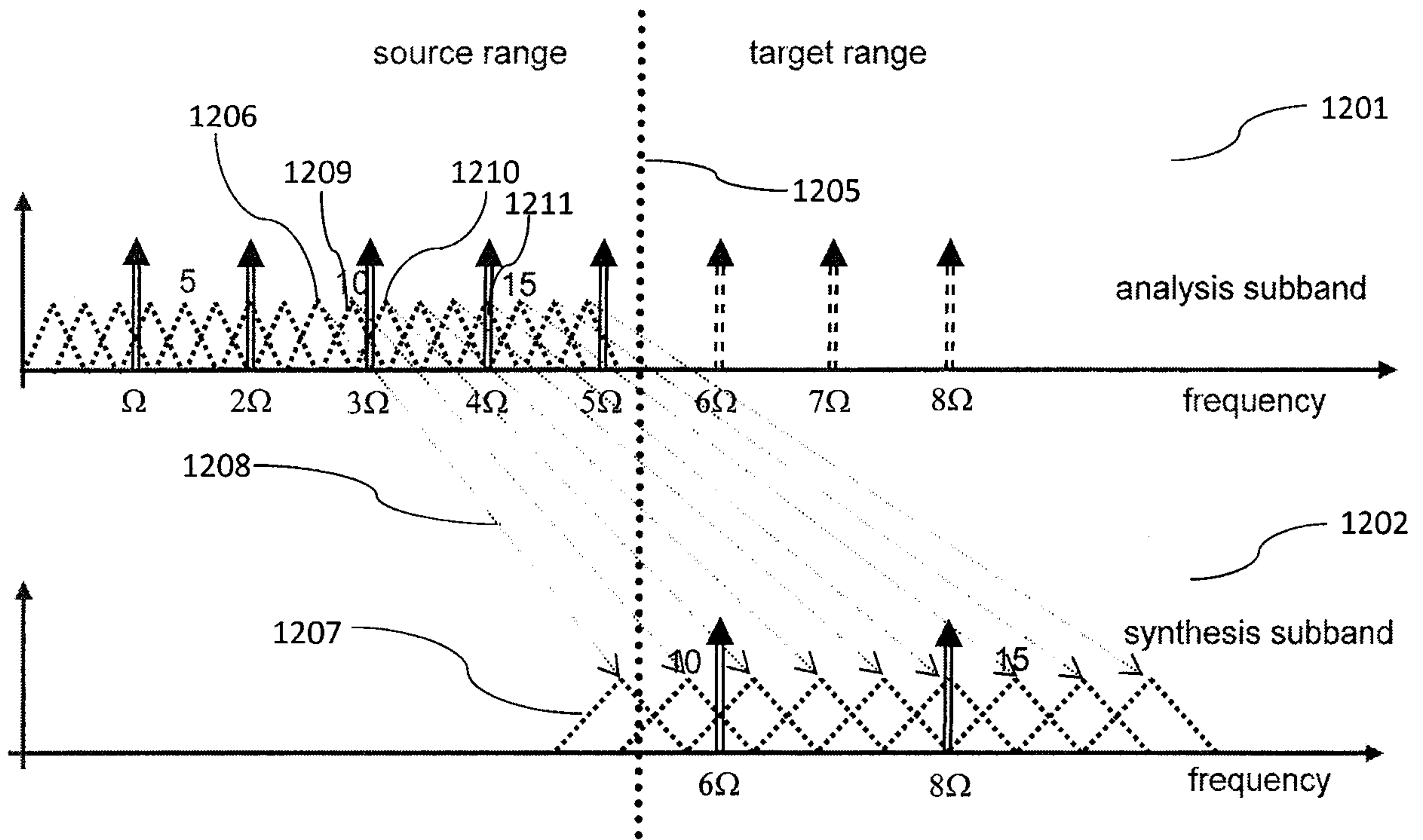
Fig. 12 - PRIOR ART
