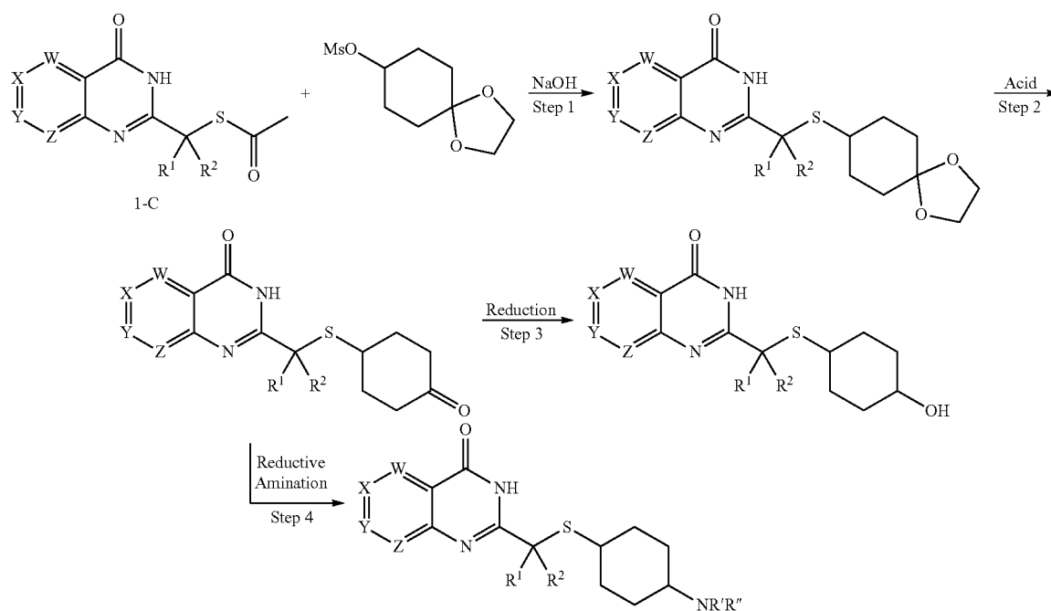
Scheme 13
