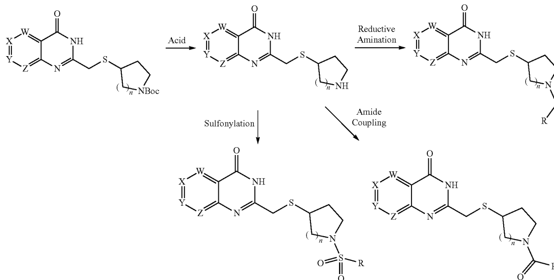
Scheme 12
