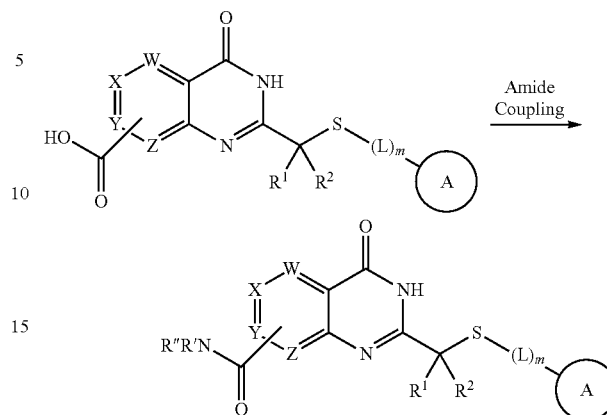
Scheme 9
