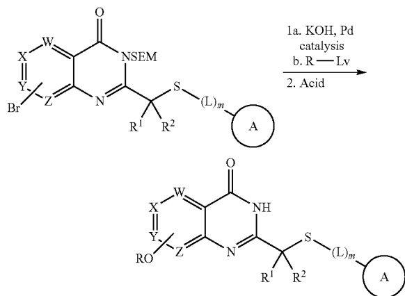
Scheme 7
