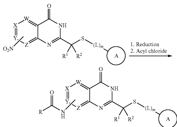
Scheme 8
