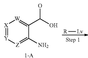
Scheme 2
