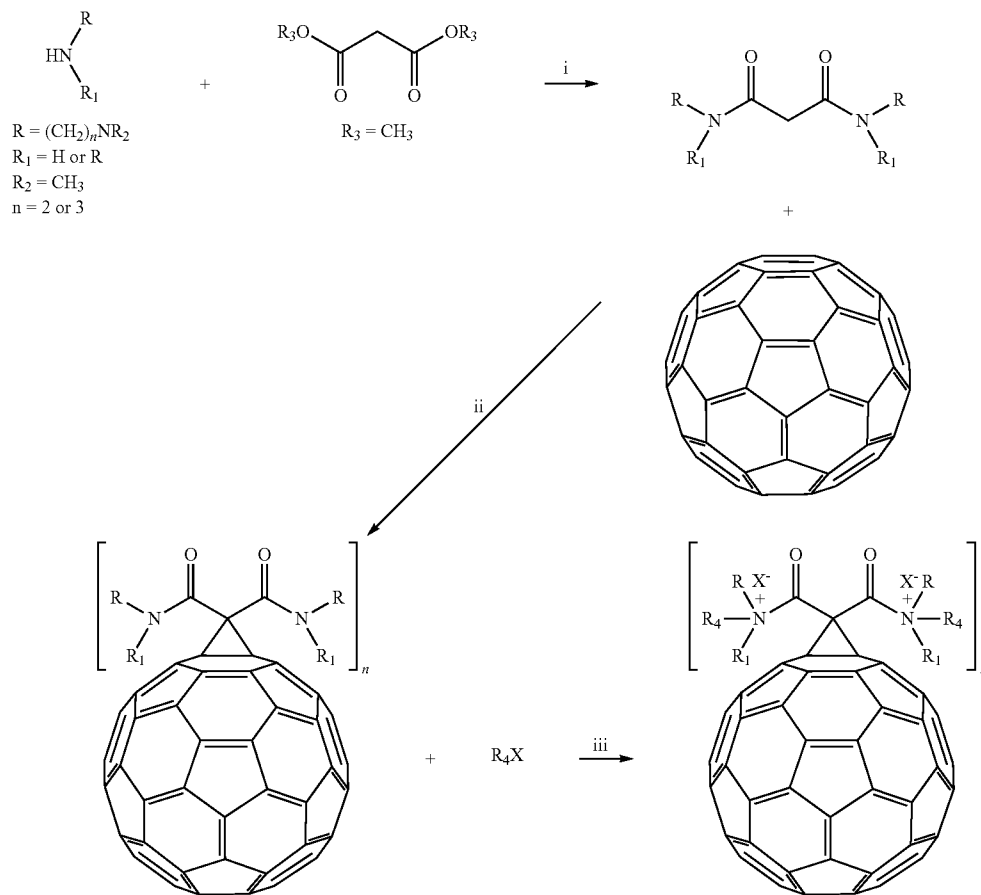
Scheme 4. Synthesis of CI4 and CI5.
