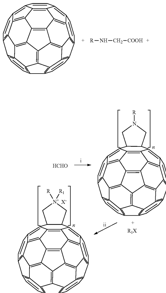
Scheme 2. Synthesis of CI1, CI2, CI3.
