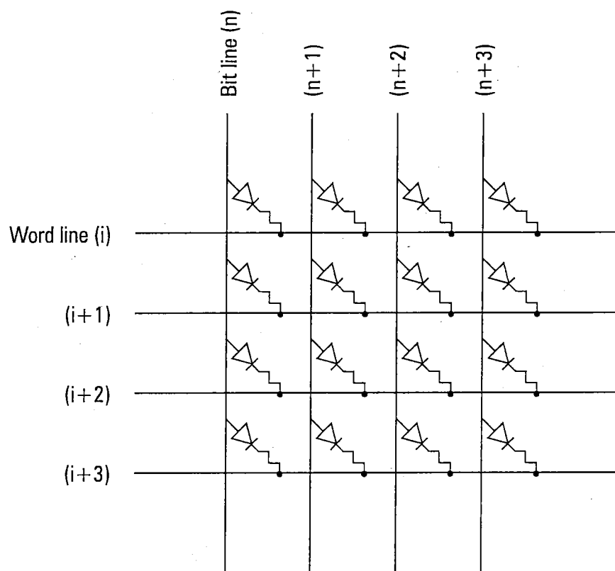
Cross Point RRAM array
