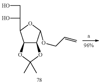
Scheme 7 Synthesis of the KDO donor
