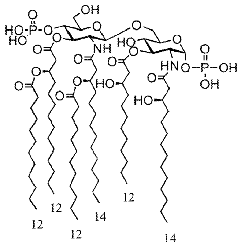
54. E. coli lipid A with shorter lipids
