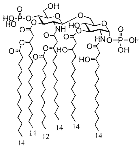
52. hexa-acylated E. coli lipid A
