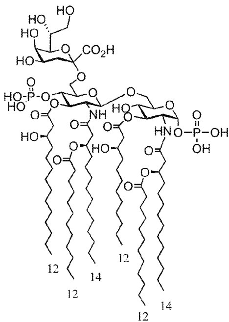
53. N. meningitidis lipid A with KDO
