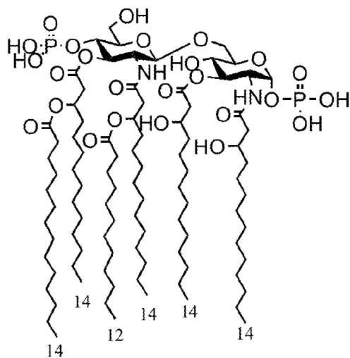
1. hexa-acylated E. coli lipid A
