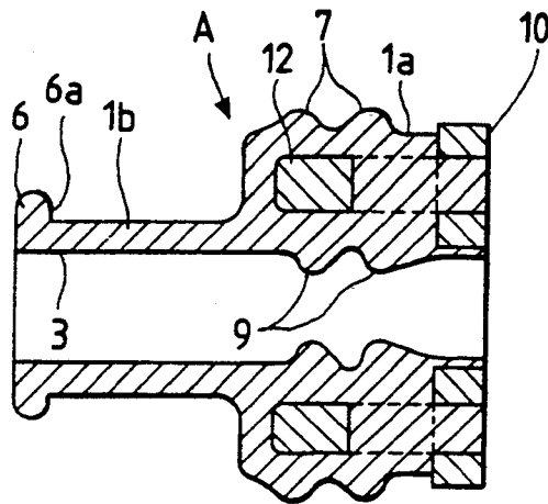
FIG. 6 PRIOR ART
