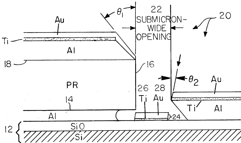
FIG. 1B. SHADOW DEPOSITION GEOMETRY.
