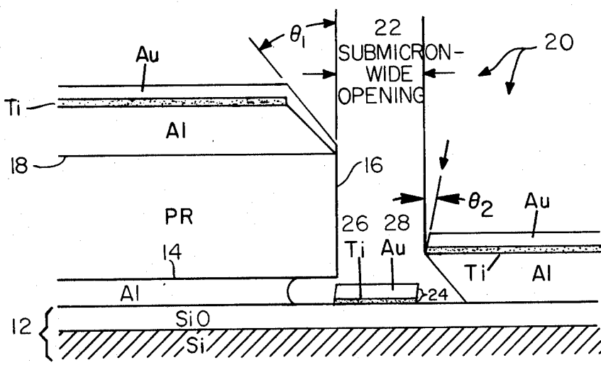
SHADOW DEPOSITION GEOMETRY.
