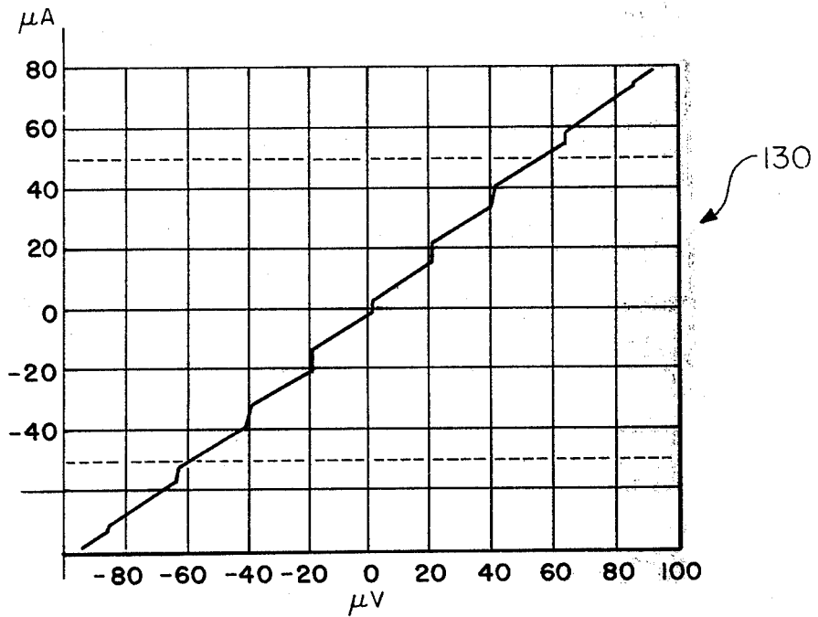
FIG. 4B. SINGLE MICROBRIDGE WITH 10 GHz RADIATION PRESENT.
