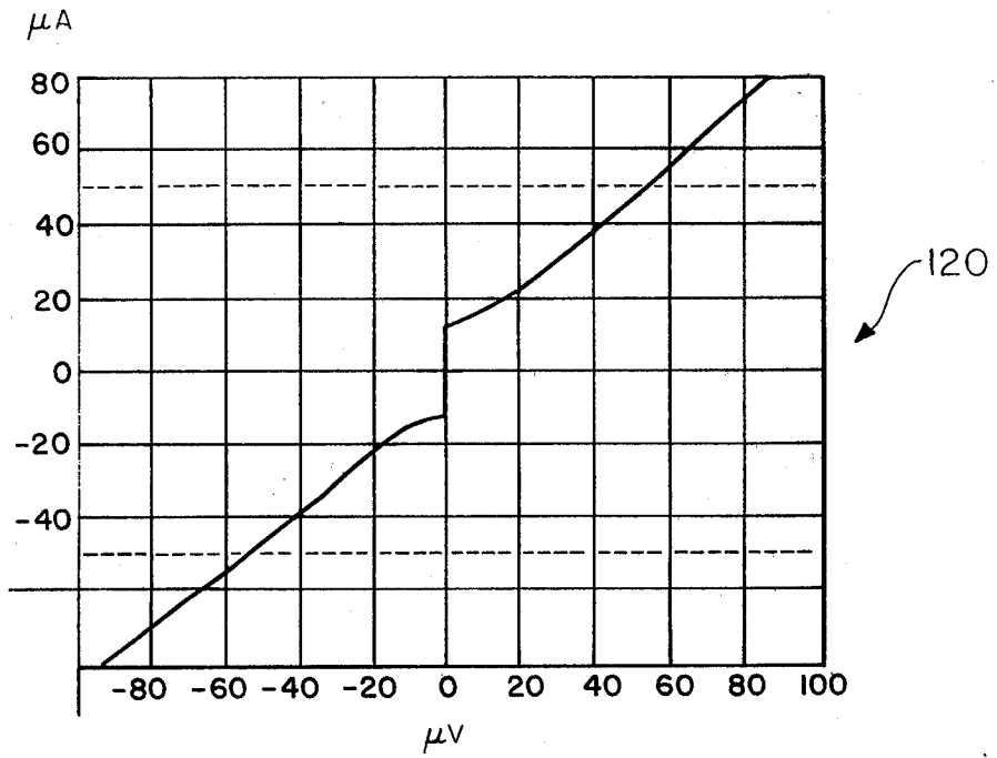
FIG. 4A. SINGLE MICROBRIDGE WITH NO APPLIED FIELDS.
