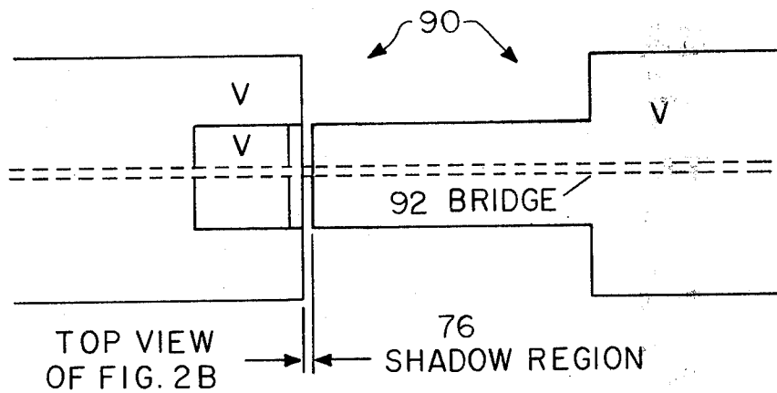
FIG. 2C. COMPLETED DEVICE (REDUCED SCALE)
