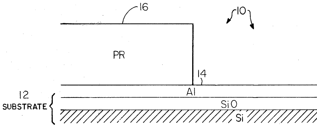
FIG. 1A. INITIAL PREPARATION OF SUBSTRATE.
