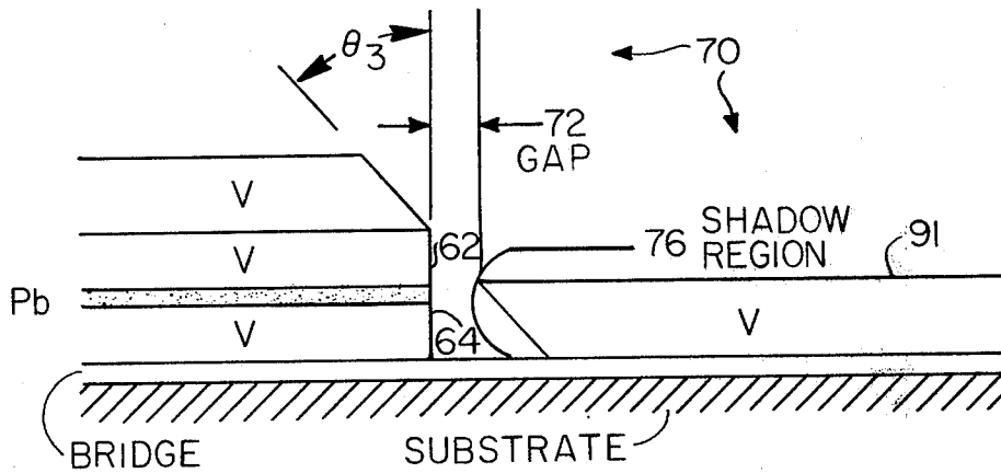
FIG. 2B. DEPOSITION OF SECOND BANK.
