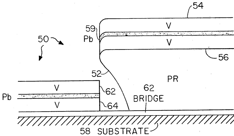
FIG. 2A. PATTERNING OF FIRST BANK.
