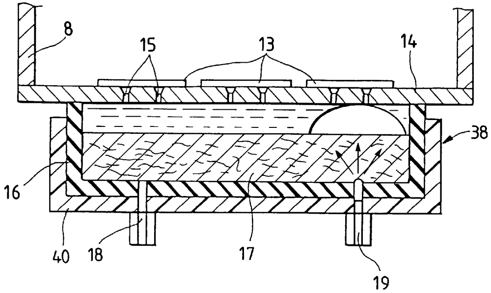
FIG. 12 PRIOR ART
