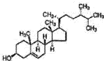
Campesterol
