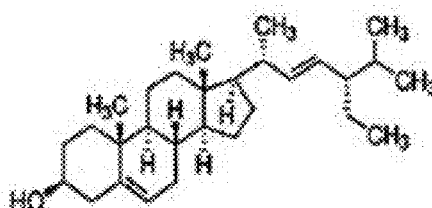
Stigmasterol
